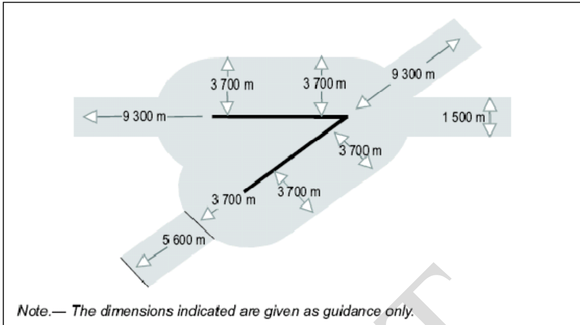
Figure 5-11. Multiple runway laser-beam free flight zone
