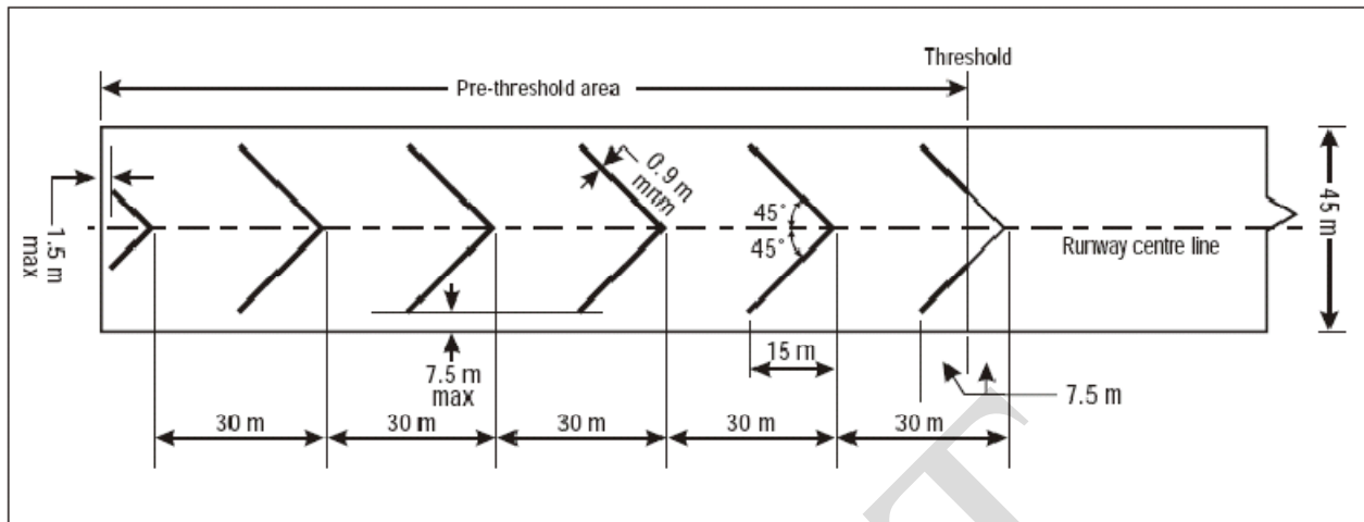
Figure 7-2. Pre-threshold marking
