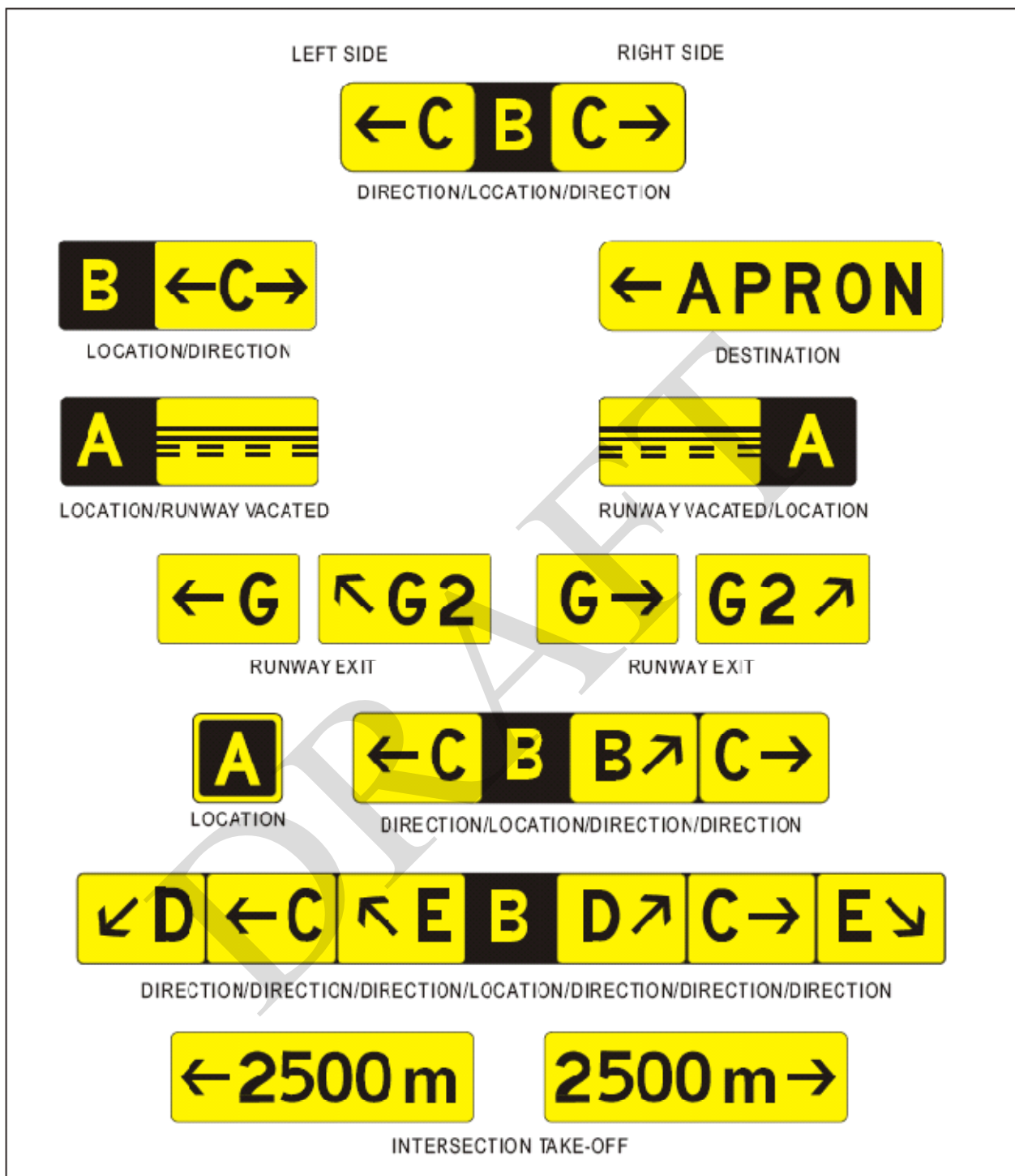
Figure 5 -28. Information signs
