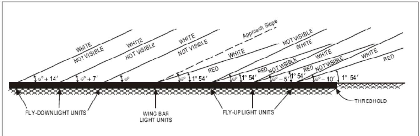
Figure 5-17. Light beams and elevation settings of T-VASIS and AT-VASIS
