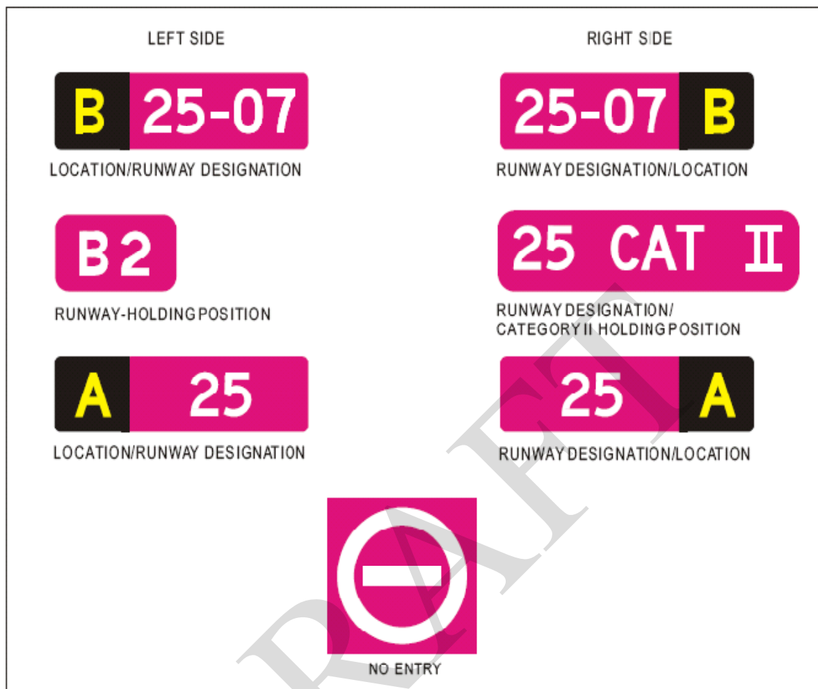
Figure 5-28 Mandatory instruction signs
