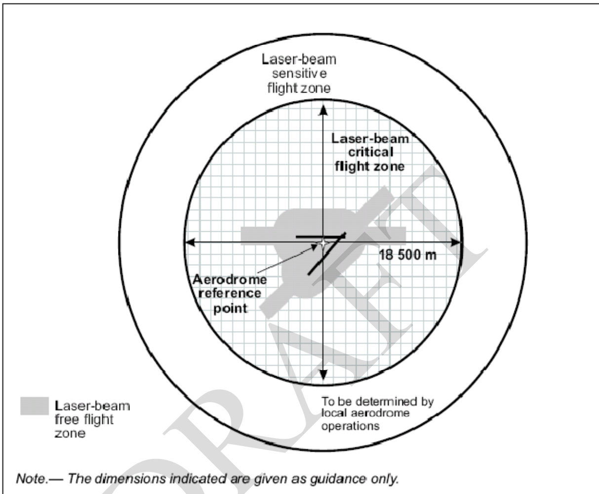
Figure 5-10. Protected flight zones
