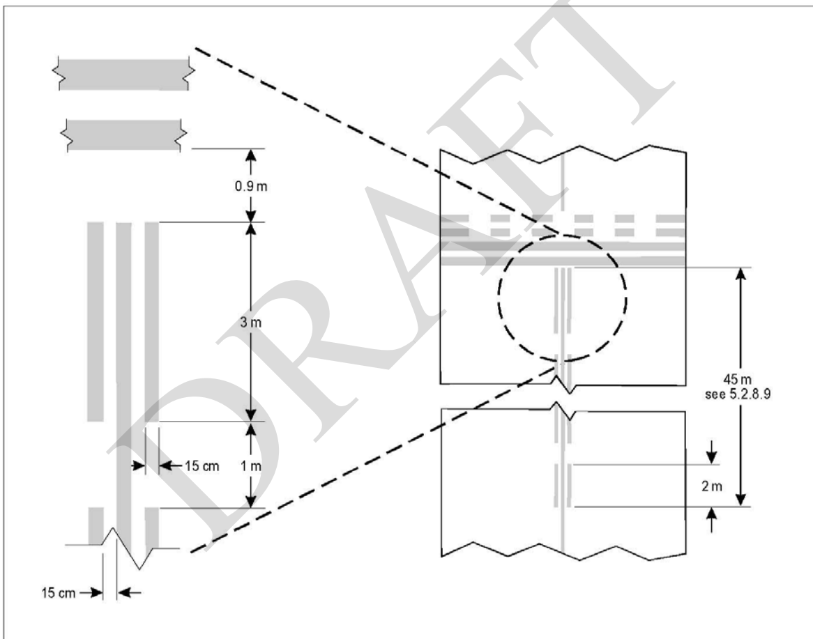
Figure 5-6A Enhanced Taxiway centre line marking
