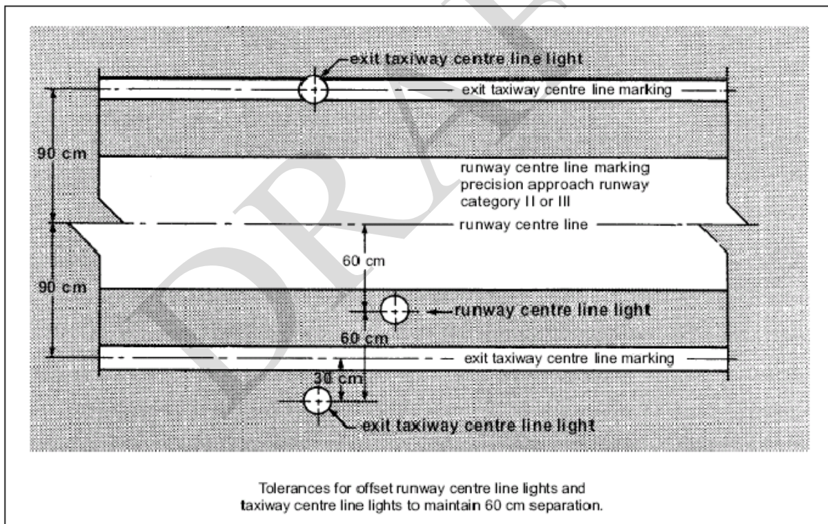
Figure 5-25. Offset runway and taxiway centre line lights
