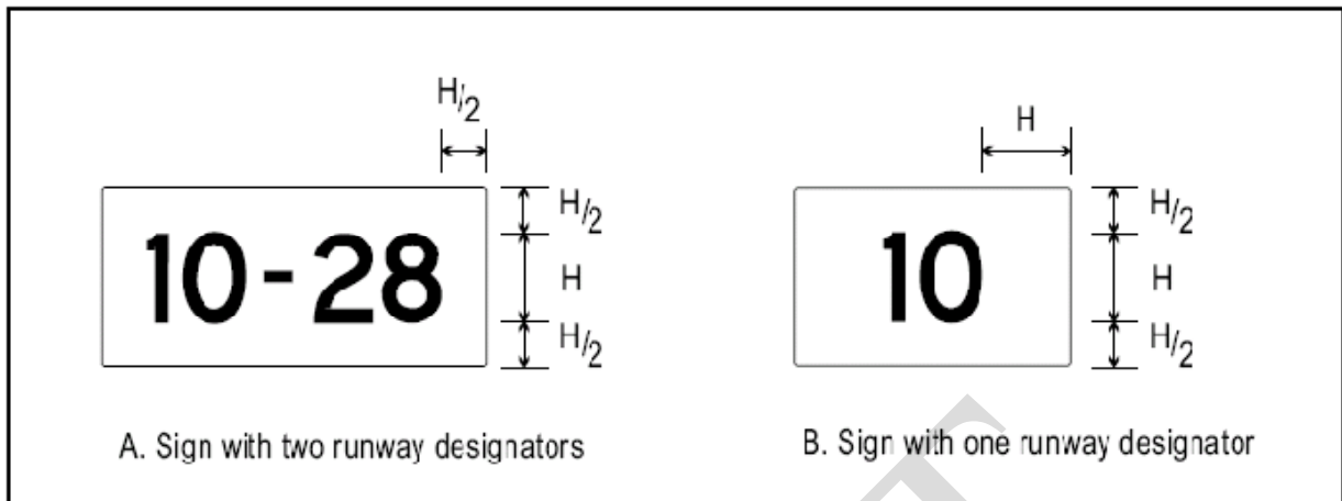
Figure A4-3. Sign dimensions
