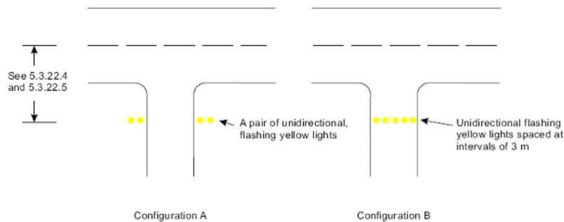
Figure 5-26 Runway guard lights
