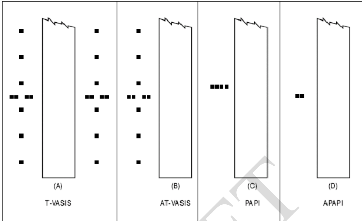
Figure 5-15. Visual approach slope indicator systems
