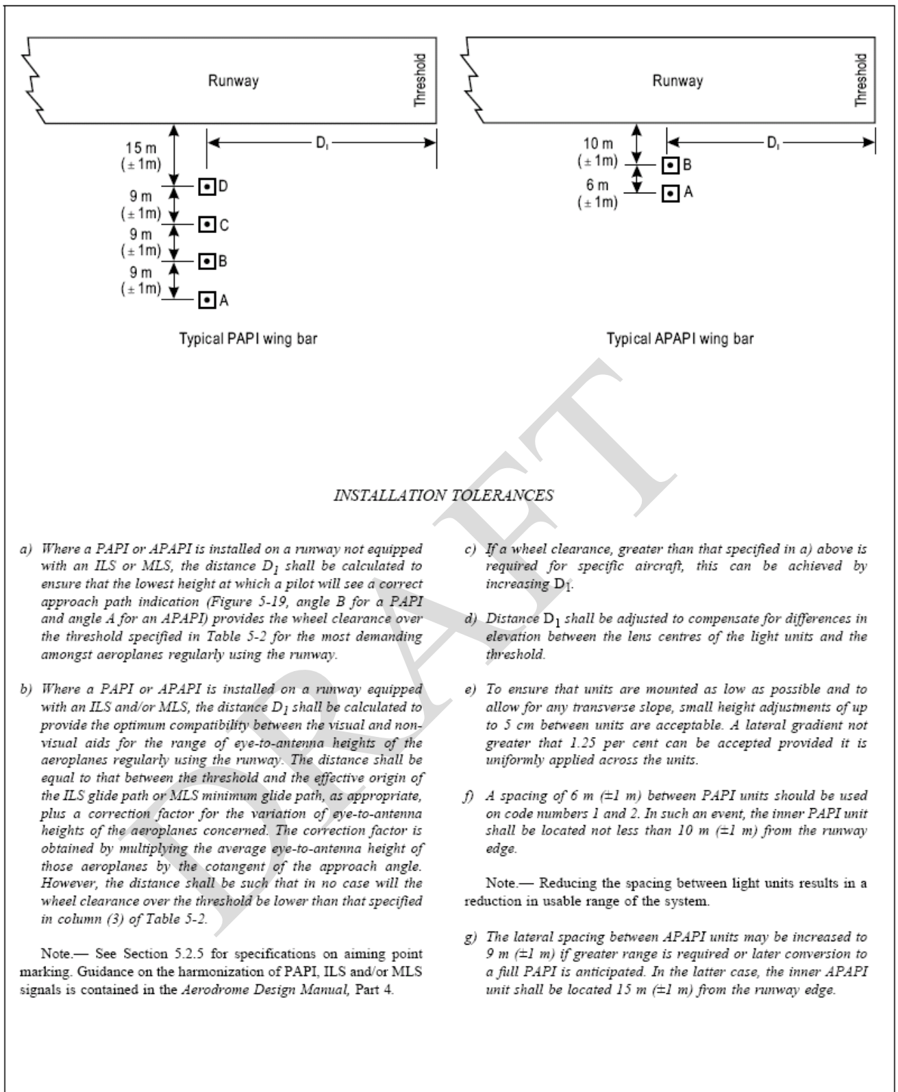
Figure 5-18. Siting of PAPI and APAPI
