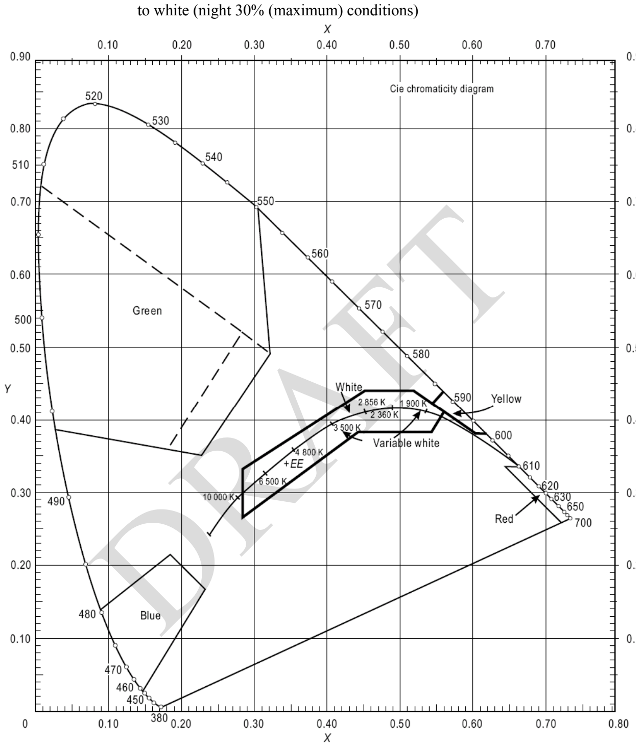
Figure A1-1. Colours for aeronautical ground lights
