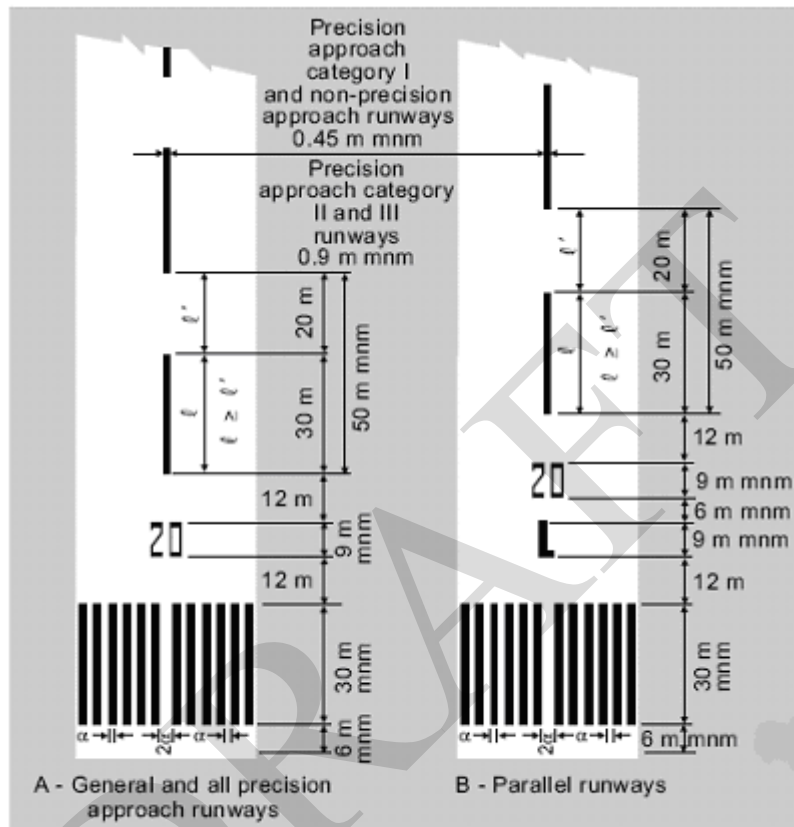
Figure 5-2. Runway designation, centre line and threshold markings
