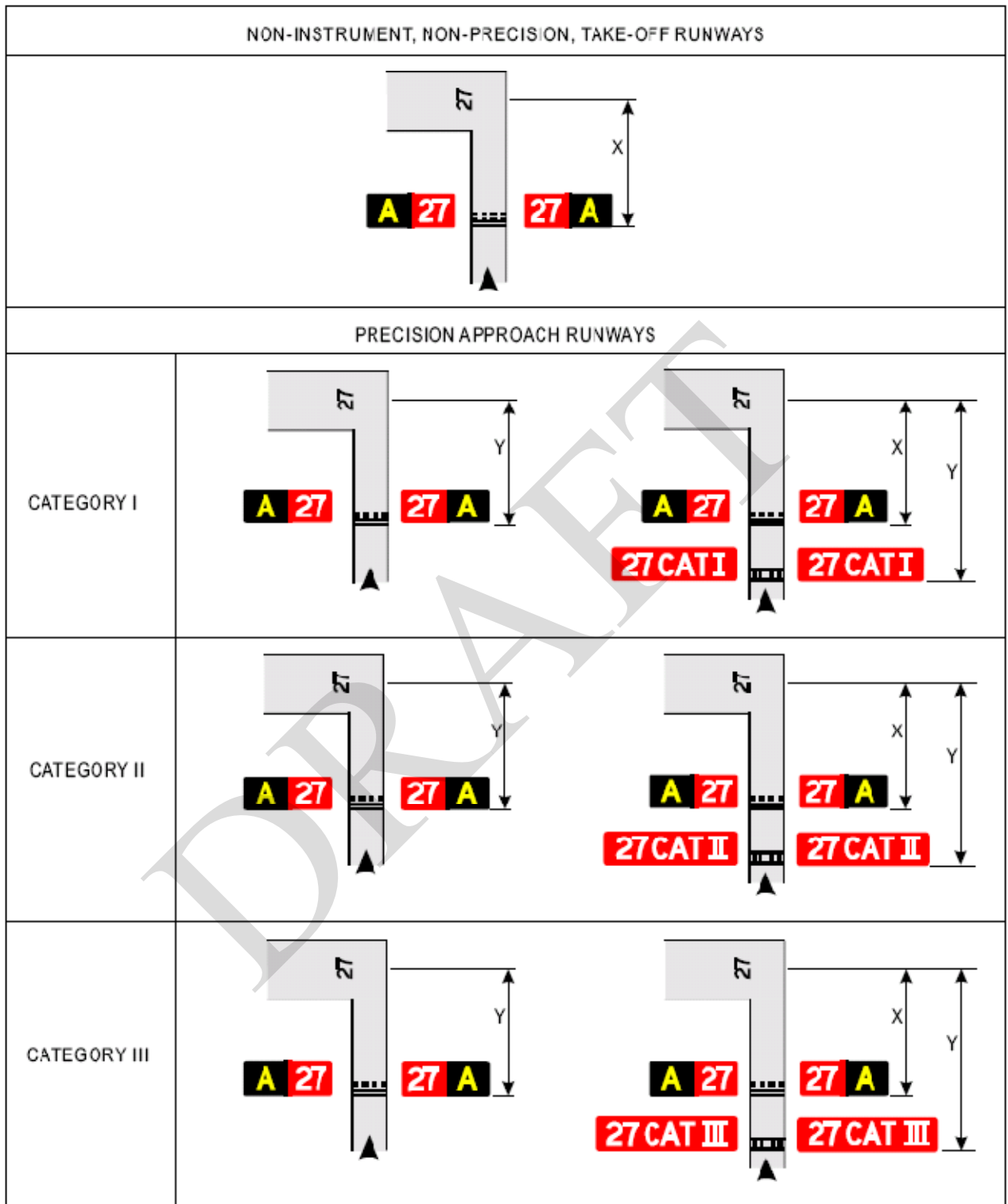
Figure 5 -29. Examples of sign positions at taxiway/runway intersections
