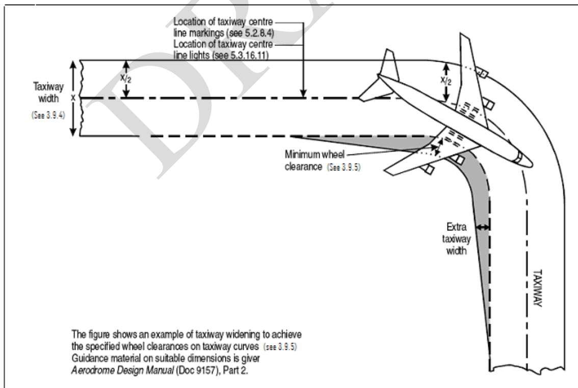
Figure 3-2. Taxiway curve
