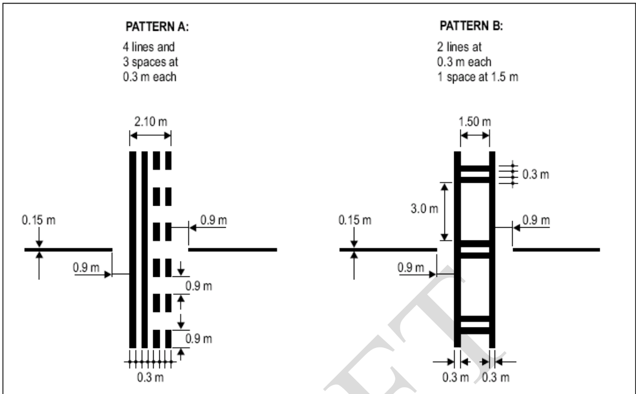
Figure 5-7. Runway-holding position markings
