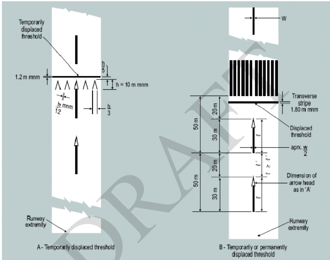
Figure 5-4. Displaced threshold markings
