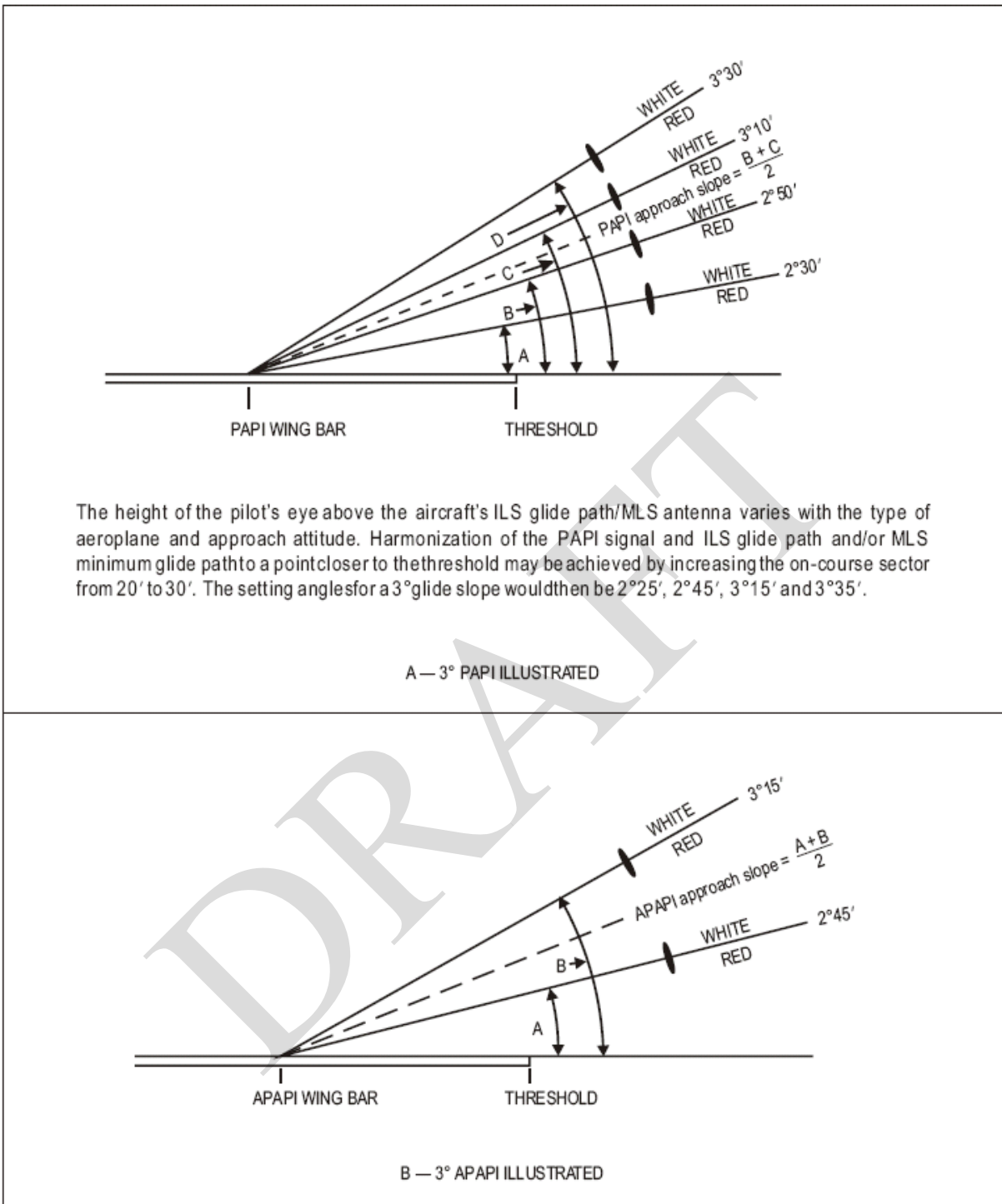
Figure 5-19. Light beams and angle of elevation setting of PAPI and APAPI
