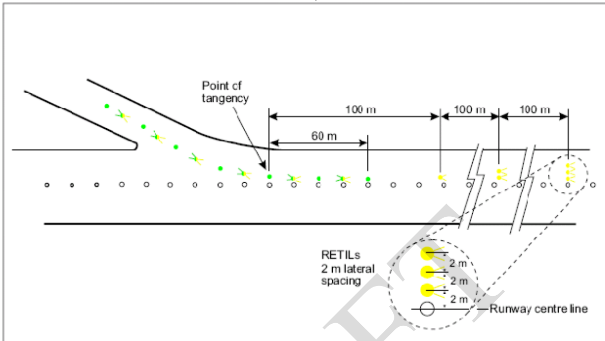
Figure 5-23. Rapid exit taxiway indicator lights (RETILs)
