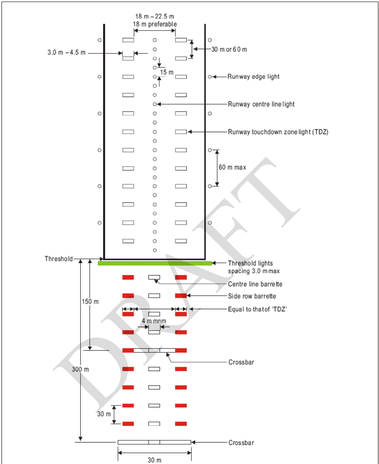
Figure 5-13. Inner 300 m approach and runway lighting for precision approach runways categories II and III
