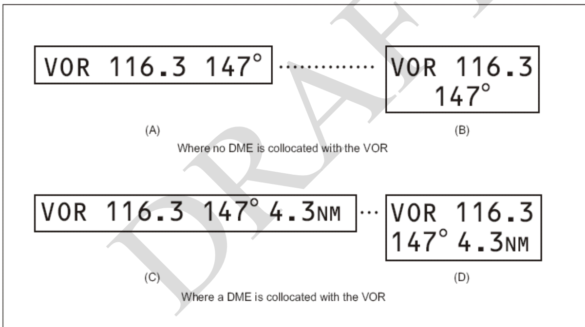
Figure 5-31. VOR aerodrome check-point sign
