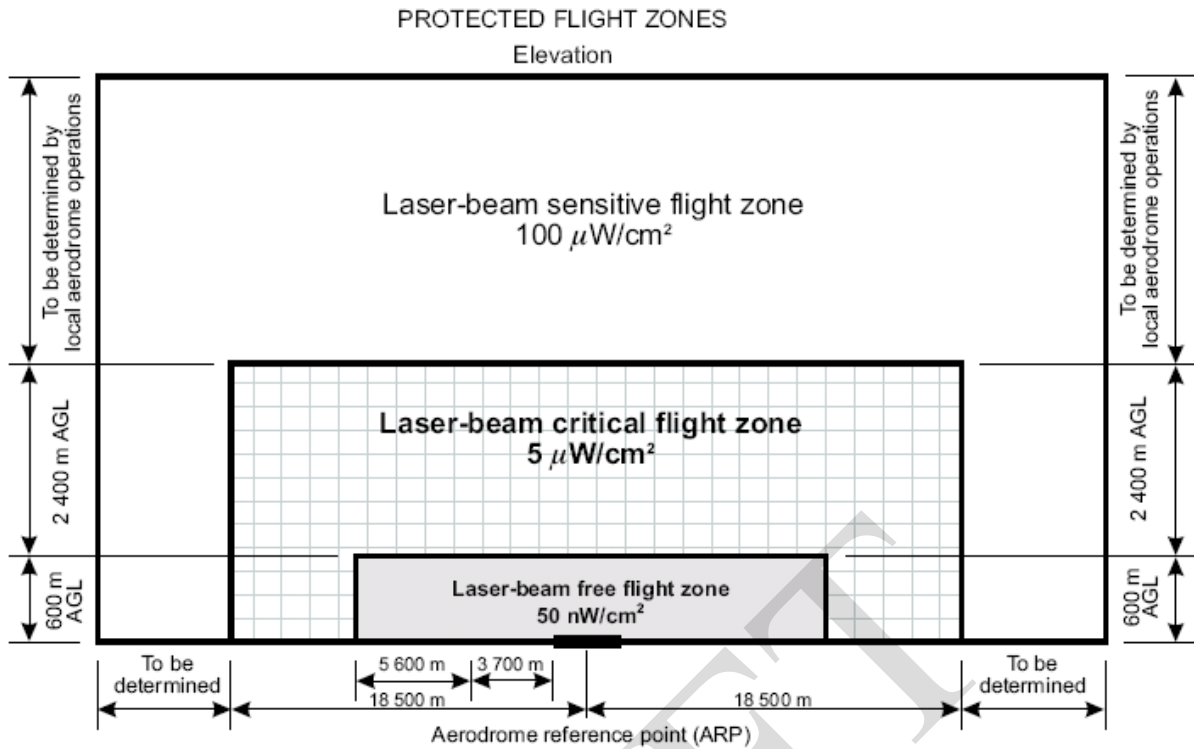
Figure 5-12. Protected flight zones with indication of maximum irradiance levels for visible laser beams
