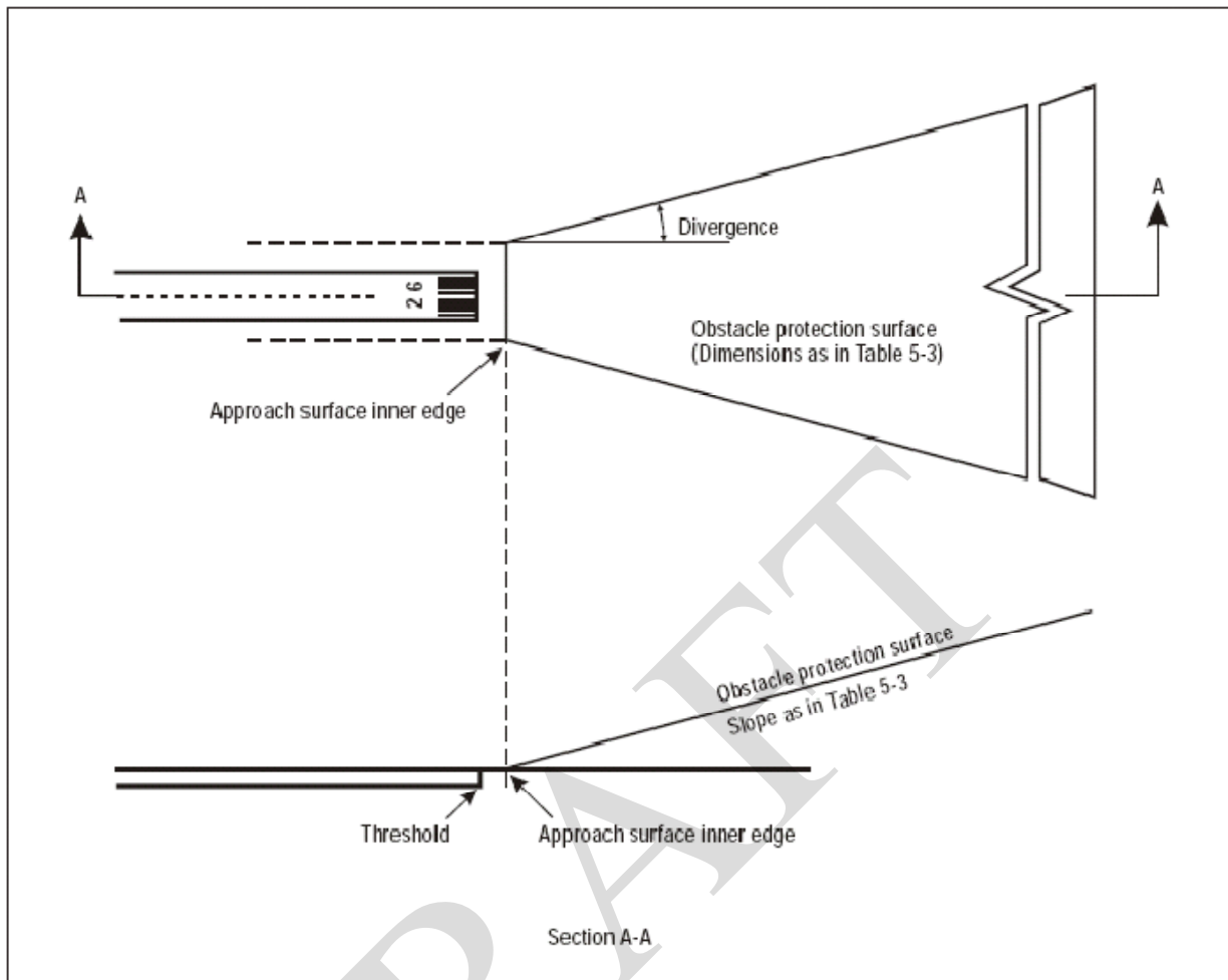
Figure 5-20. Obstacle protection surface for visual approach slope indicator systems
