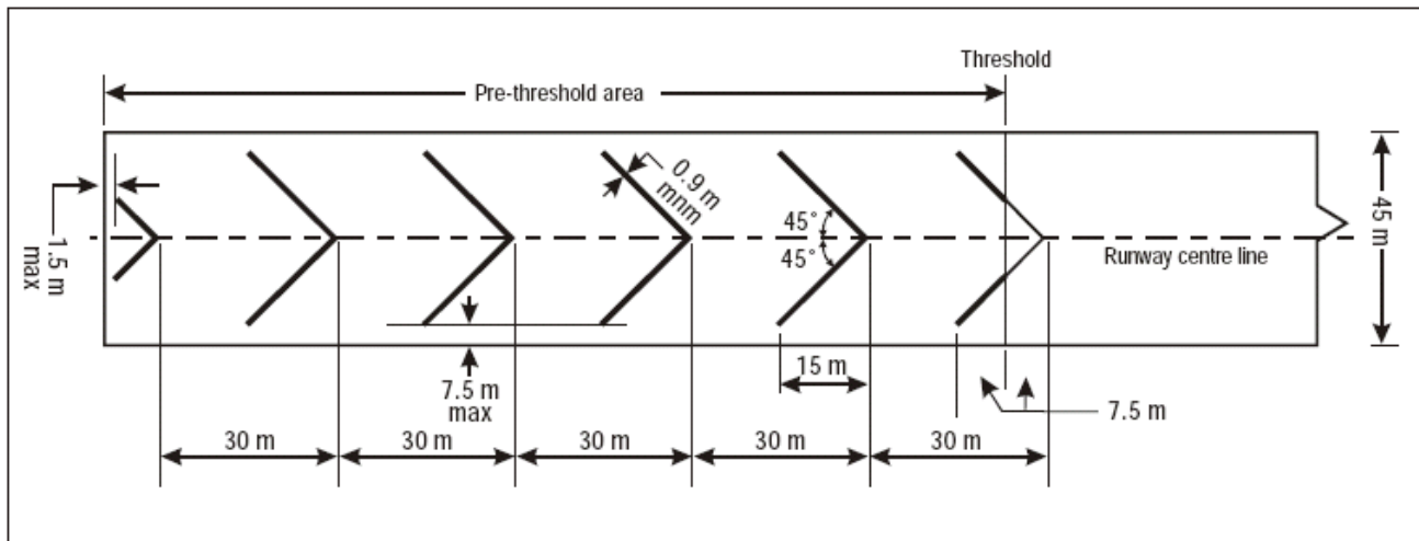
Figure 7-2. Pre-threshold marking
