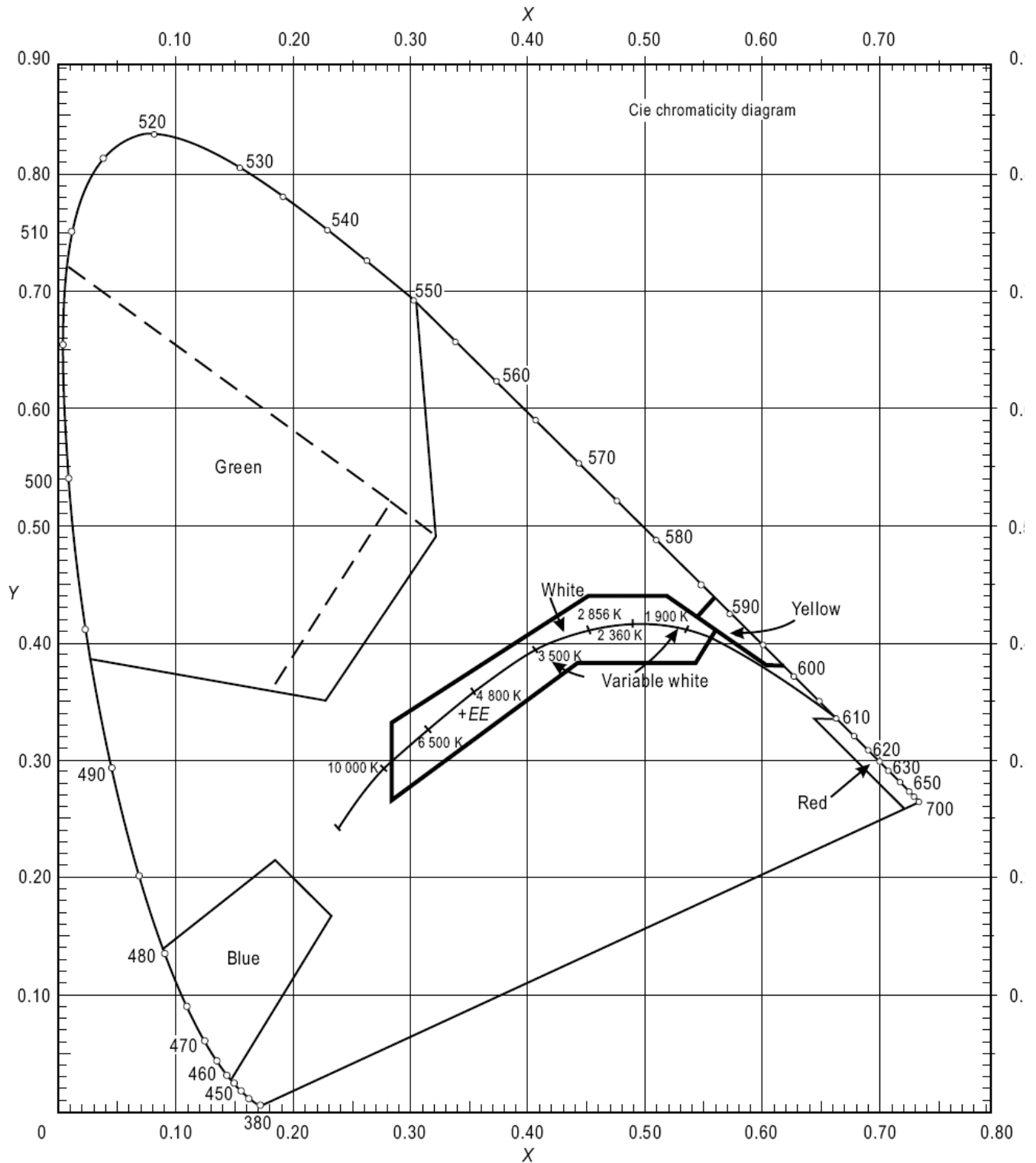
Figure A1-1. Colours for aeronautical ground lights
