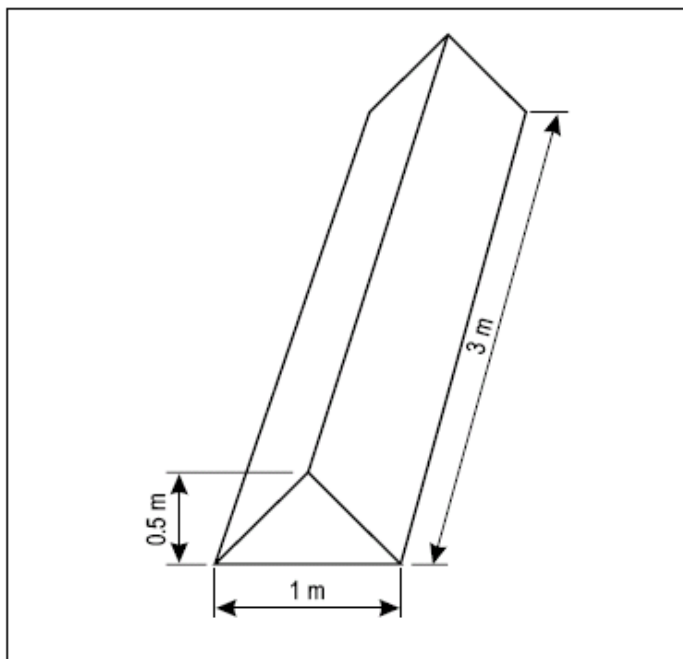
Figure 5 -28. Boundary markers
