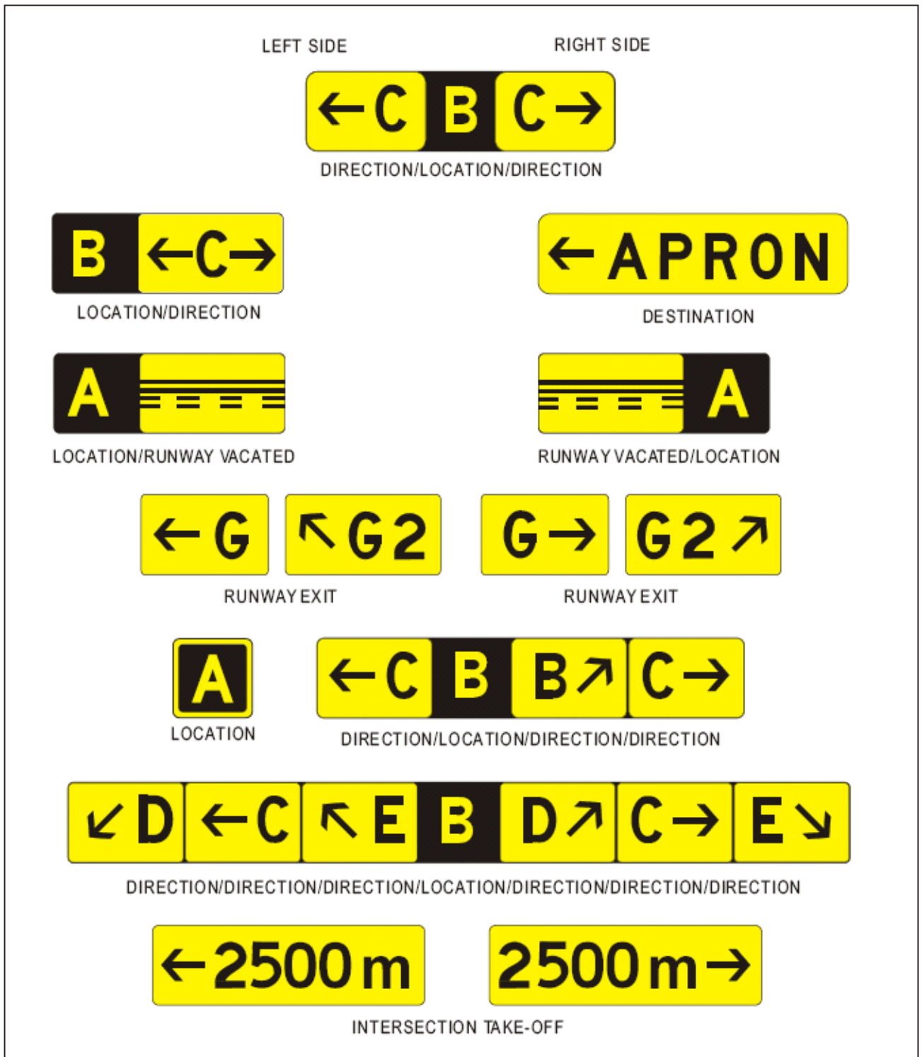
Figure 5 -28. Information signs
