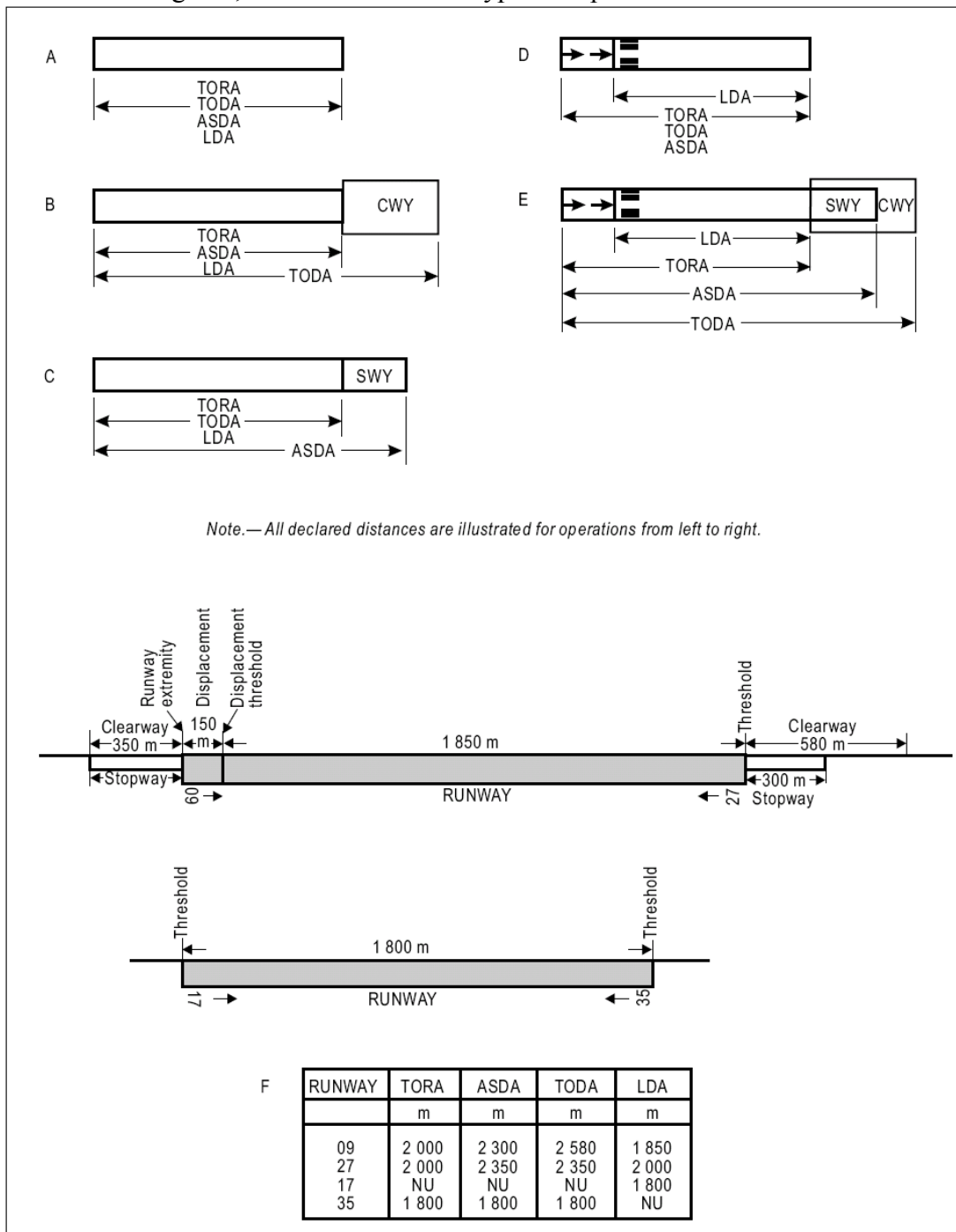
Figure A-1. Illustration of declared distances
