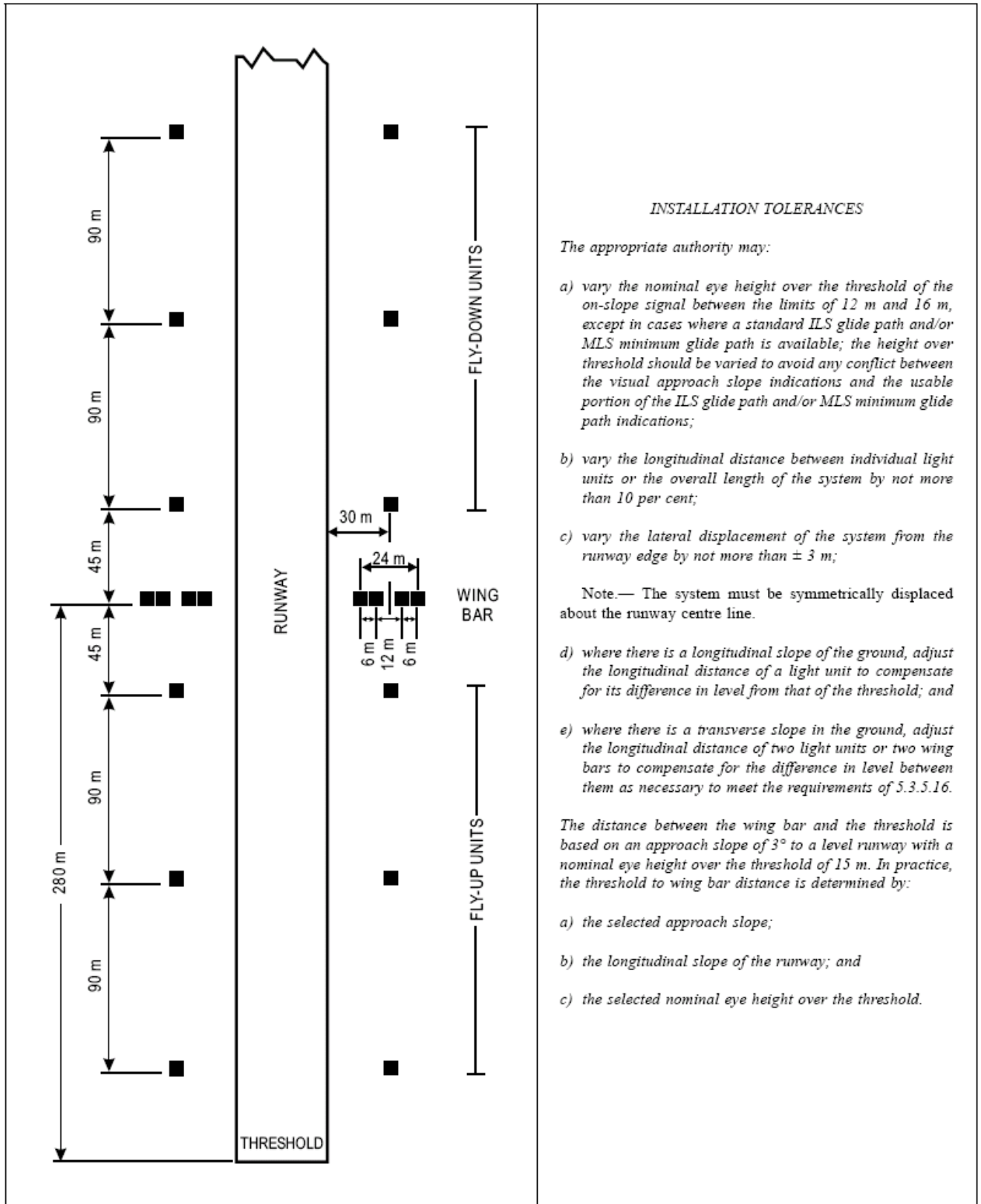
Figure 5-16. Siting of light units for T-VASIS
