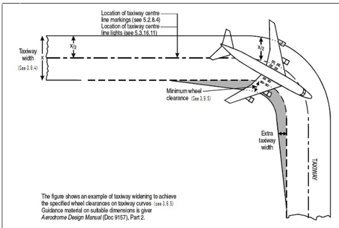
Figure 3-2. Taxiway curve
