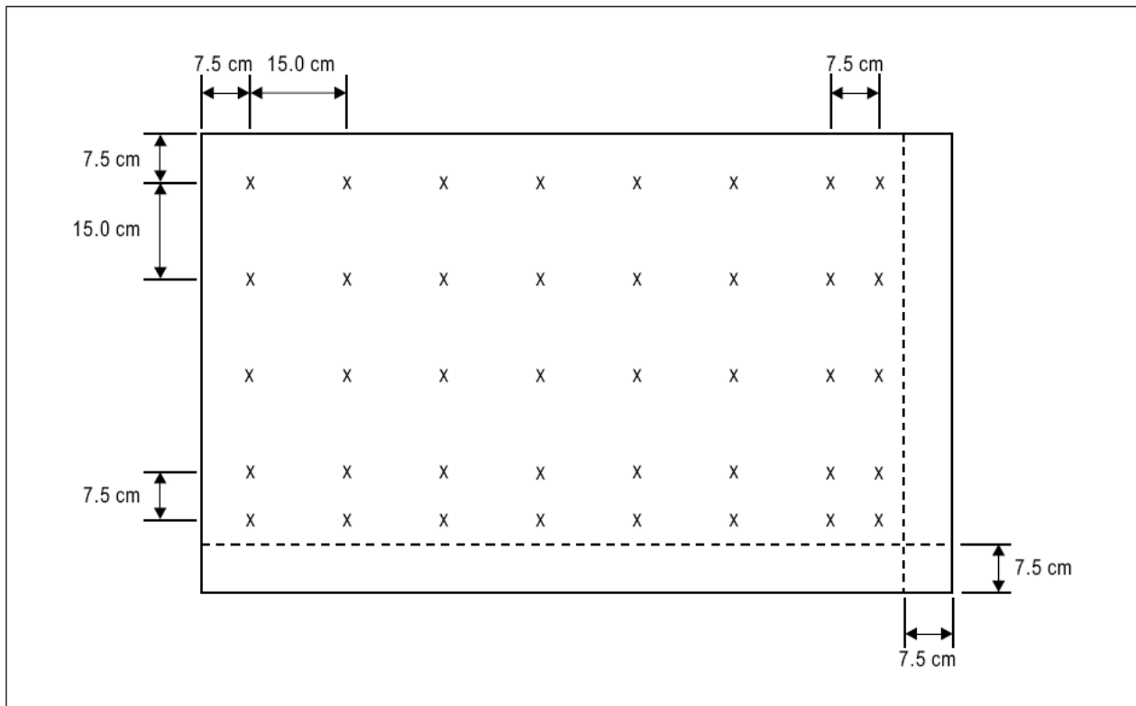
Figure A4-1. Grid points for calculating average luminance of a sign
