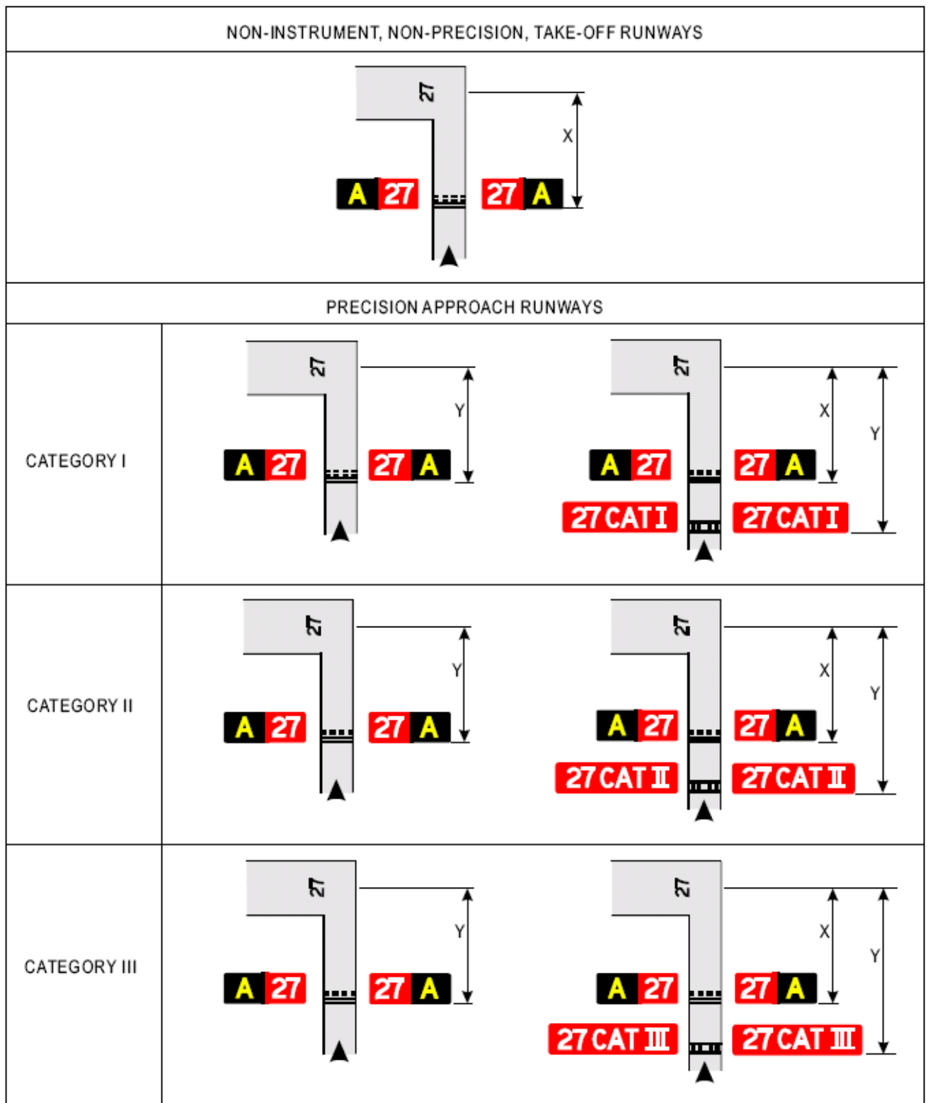
Figure 5 -29. Examples of sign positions at taxiway/runway intersections
