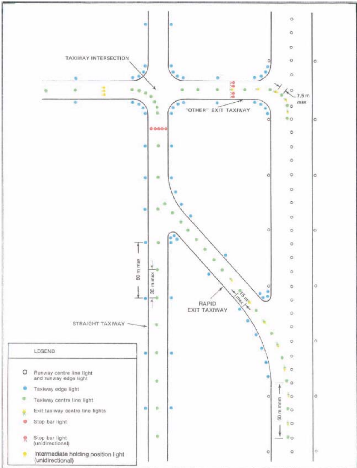
Figure 5-24. Taxiway lighting
