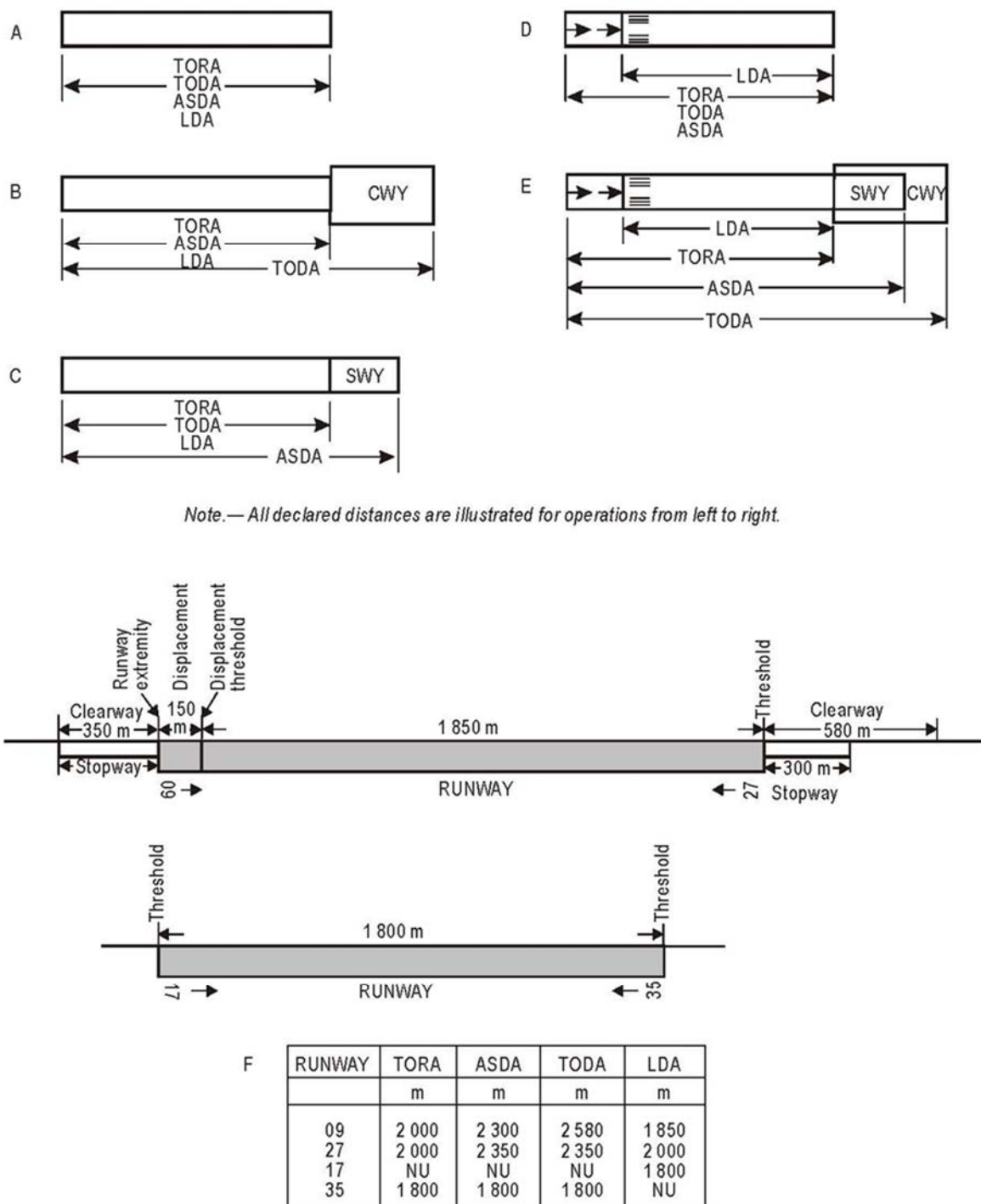
Figure A-I Illustration of declared distances
