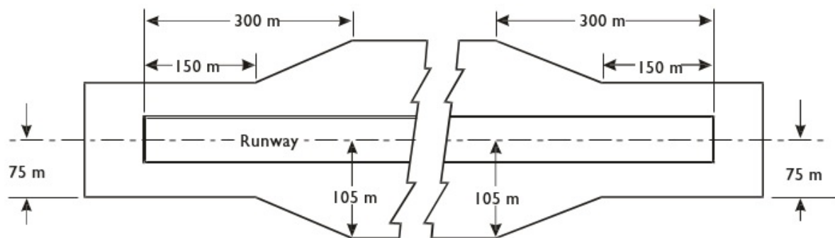
Figure A-4. Graded portion of a strip including a precision approach runway where the code number is 3 or 4
