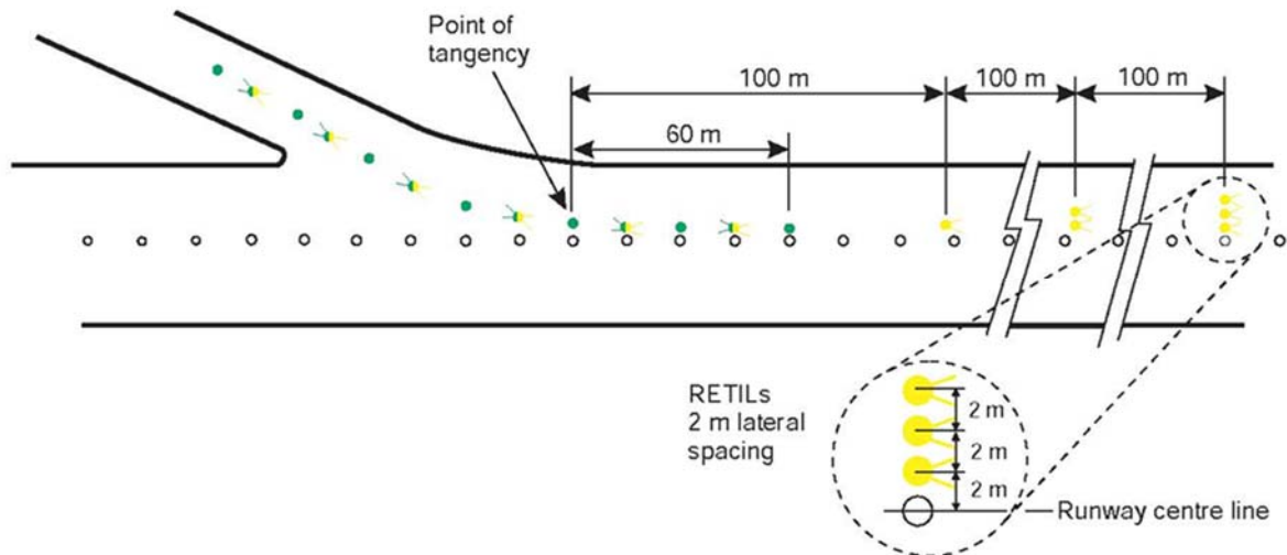
Figure 5-25 Rapid exit taxiway indicator lights (RETILS)
