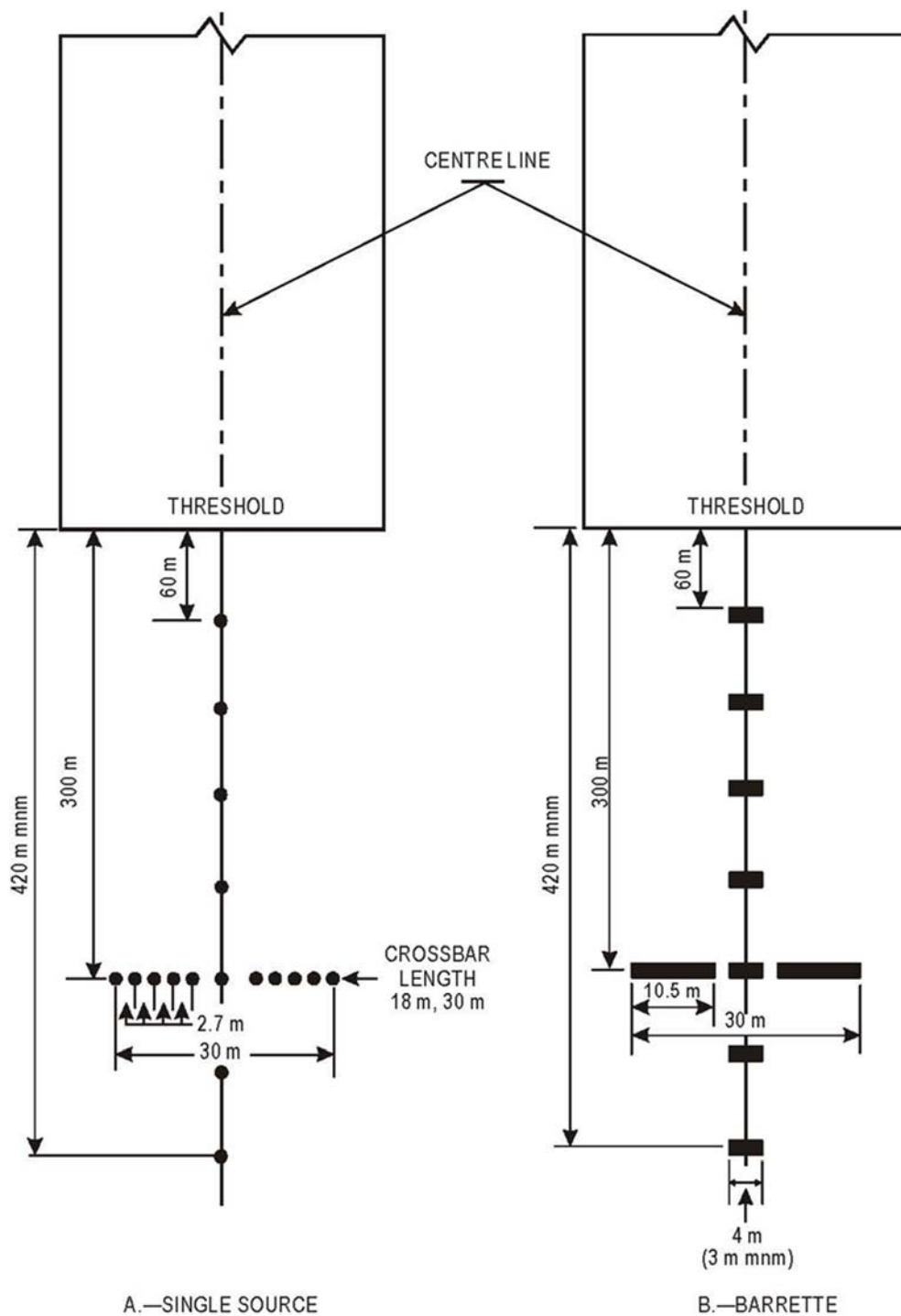
Figure A-7. Simple approach lighting systems
