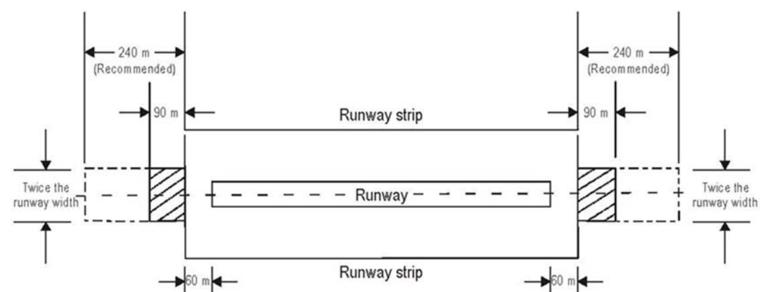
Figure A-5. Runway end safety area for a runway where the code number is 3 or 4
