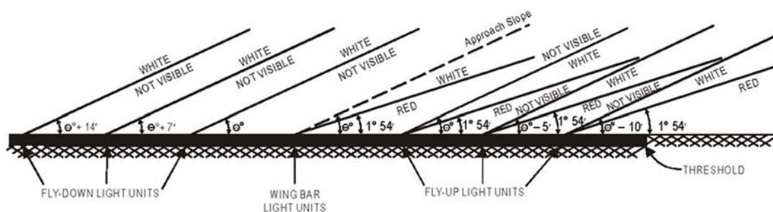
Figure 5-8 Light beams and elevation settings of T-VASIS and AT-VASIS
