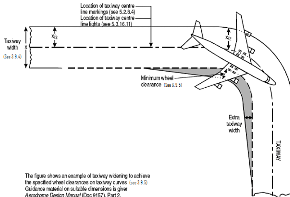
Figure 3-2 Taxiway curve
