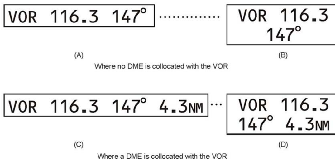
Figure 5-33 VOR aerodrome checkpoint sign
