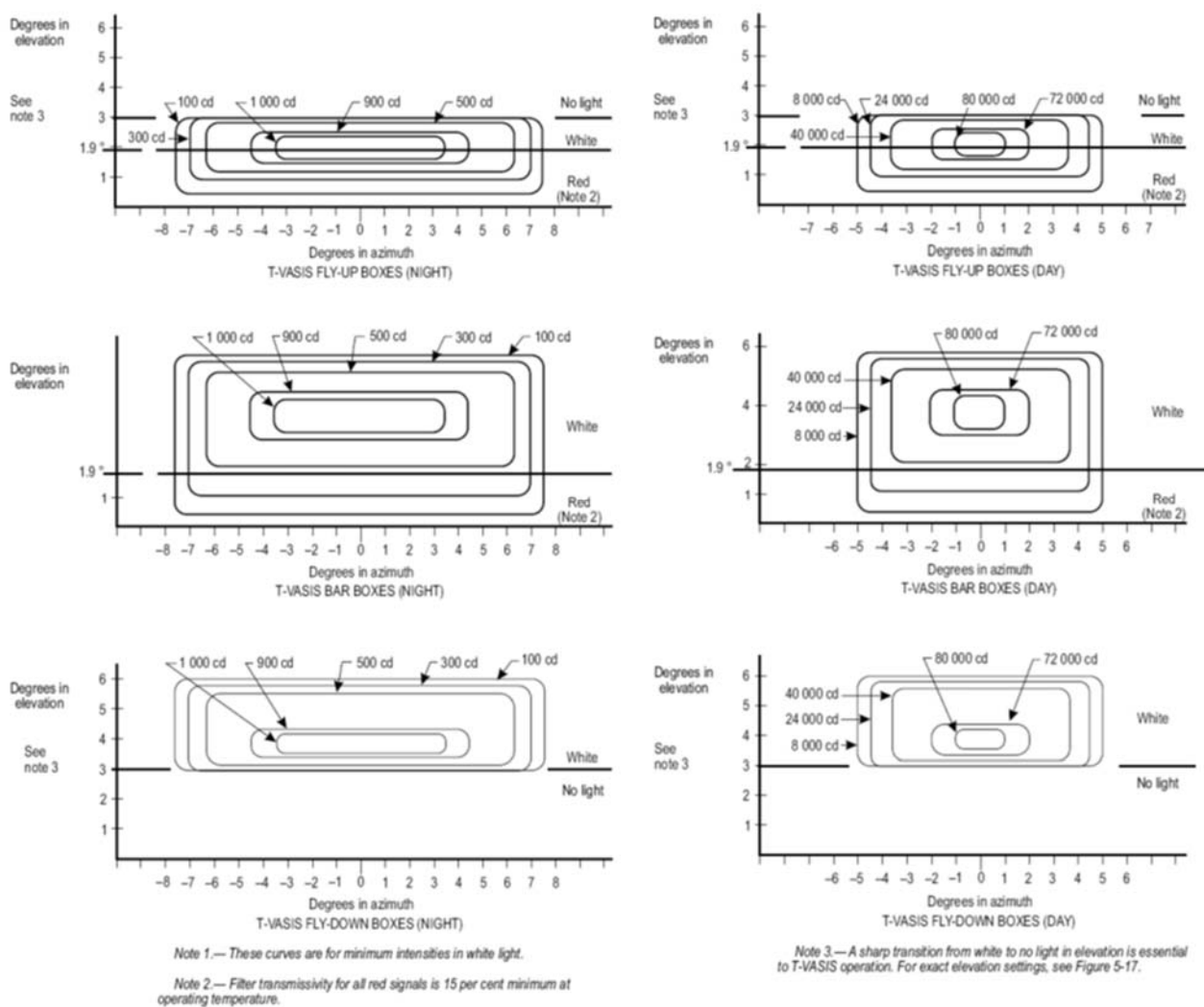
Figure A2-22 Light intensity distribution of T-VASIS and AT-VASIS
