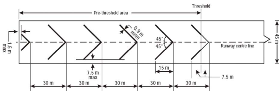
Figure 7-2 Pre-threshold marking
