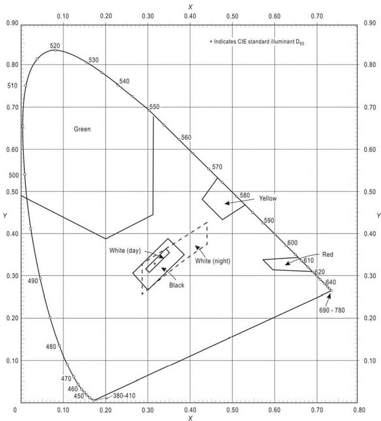
Figure AI-4 Colours of luminescent or transilluminated (internally illuminated) signs and panels
