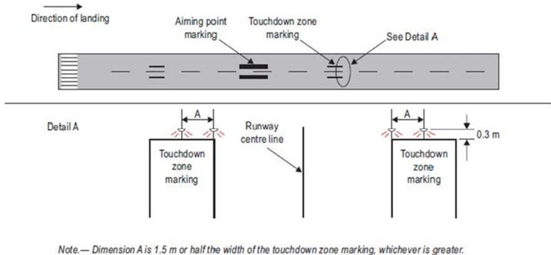
Figure 5-24 Simple touchdown zone lighting
