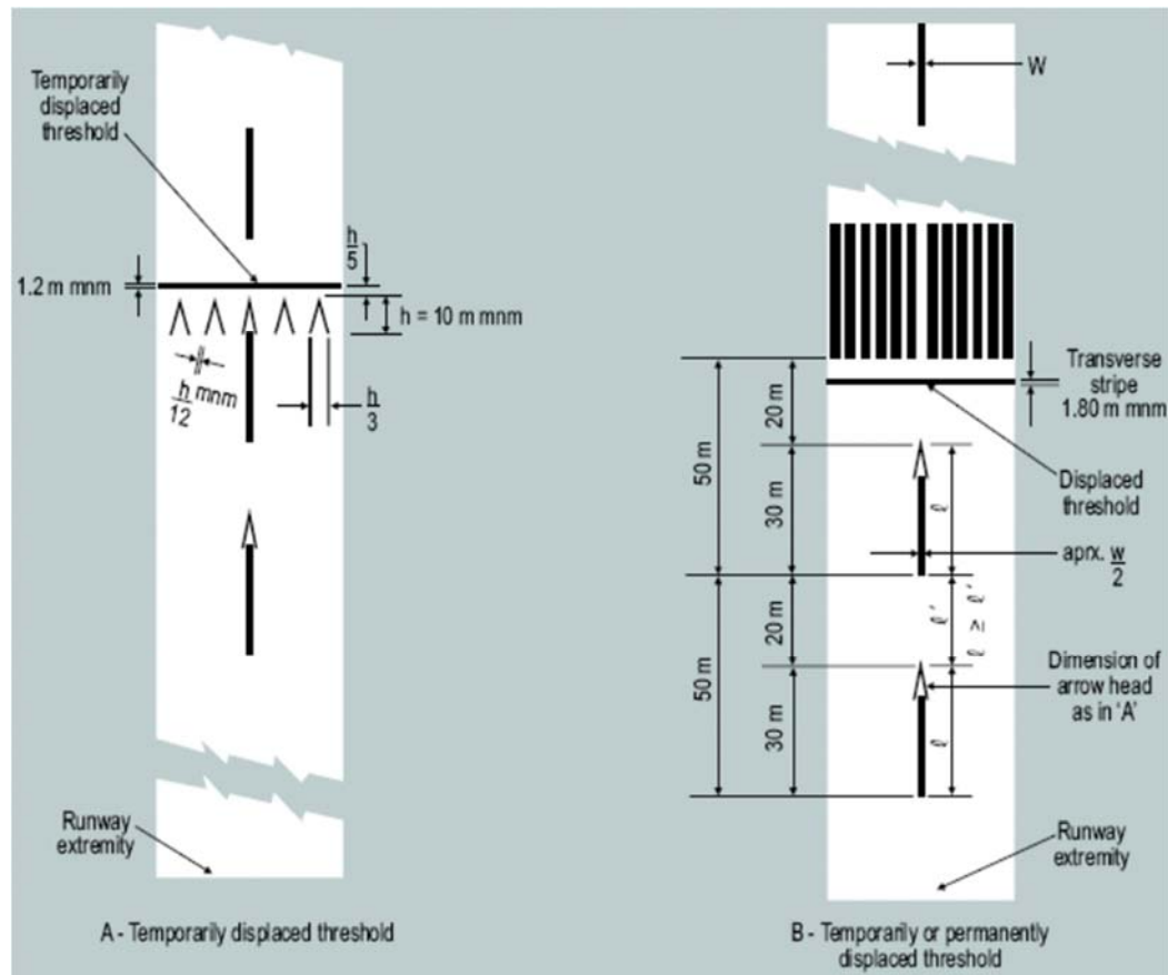
Figure 5-4 Displaced threshold markings
