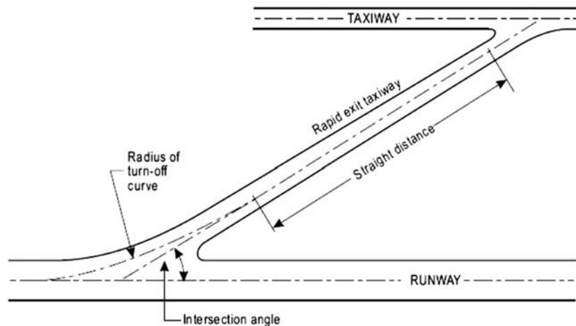
Figure 3-3 Rapid exit taxiway
