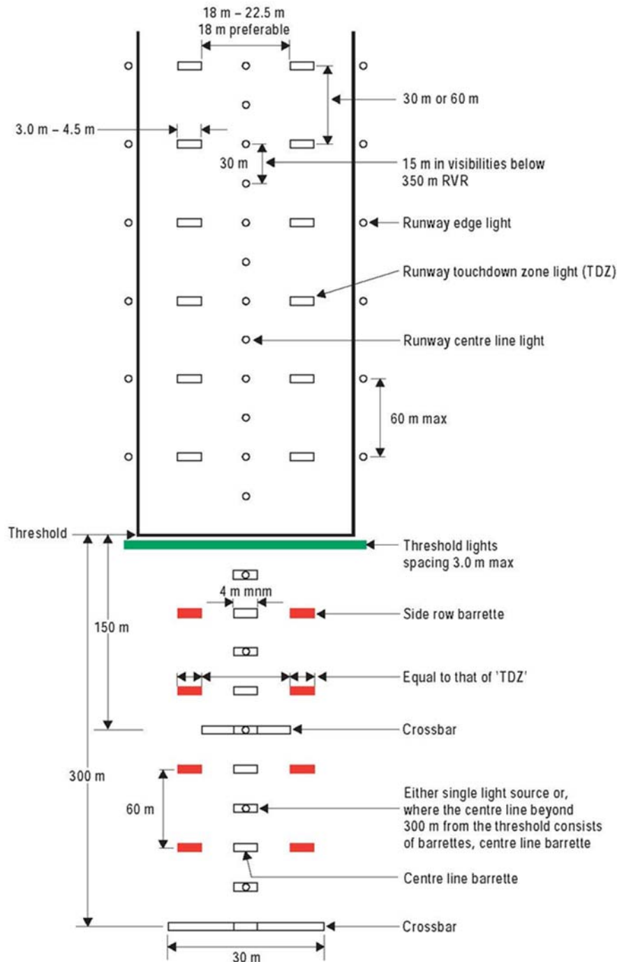
Figure 5-15 Inner 300 m approach and runway lighting for precision approach runways, categories II and III where the serviceability of the lights specified as maintenance objectives in Chapter 10 can be demonstrated
