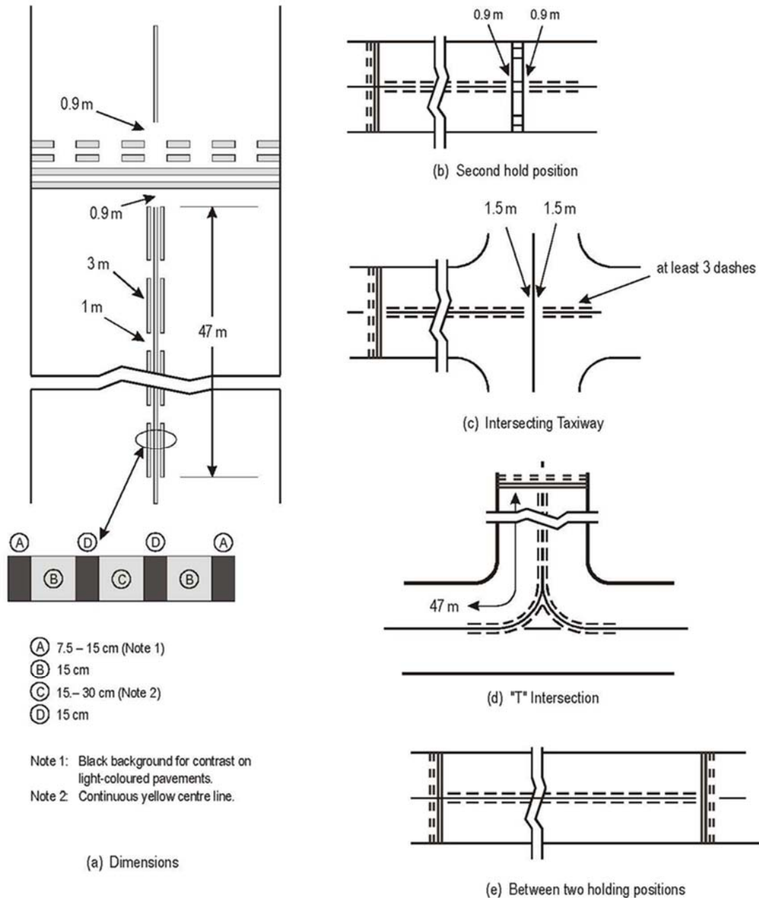
Figure 5-7 Enhanced taxiway centre line marking
