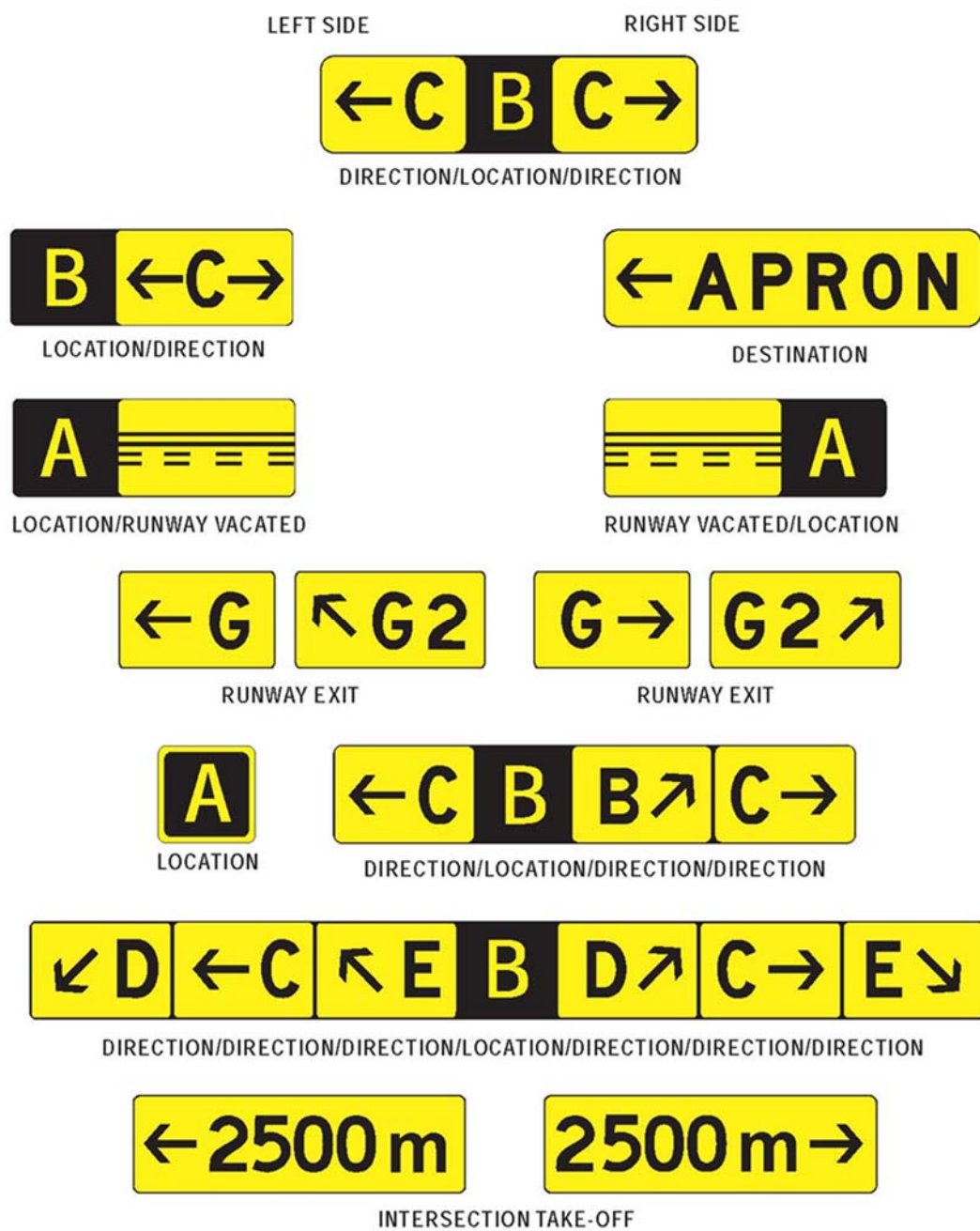
Figure 5-31 Information signs
