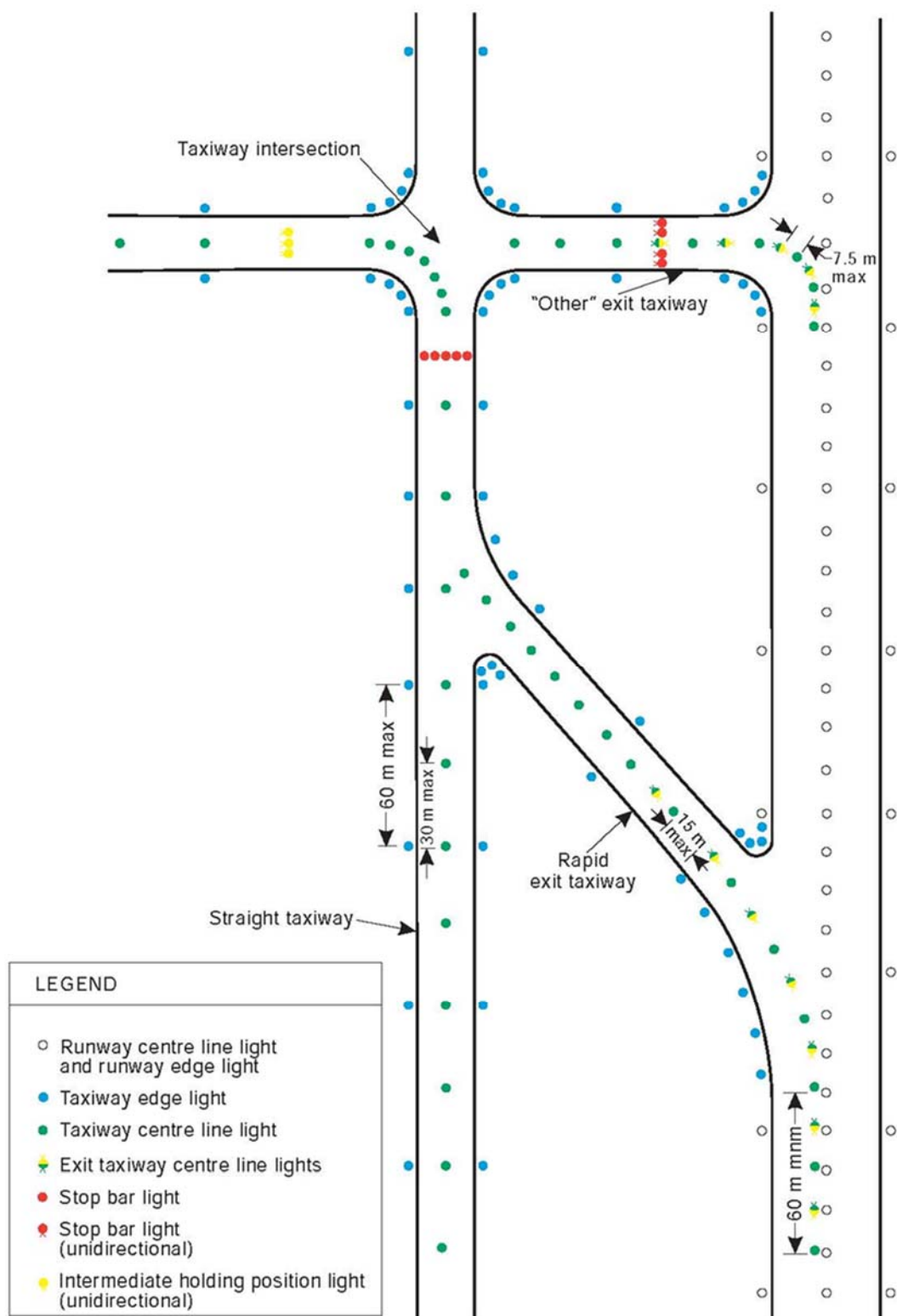
Figure 5-26 Taxiway lighting
