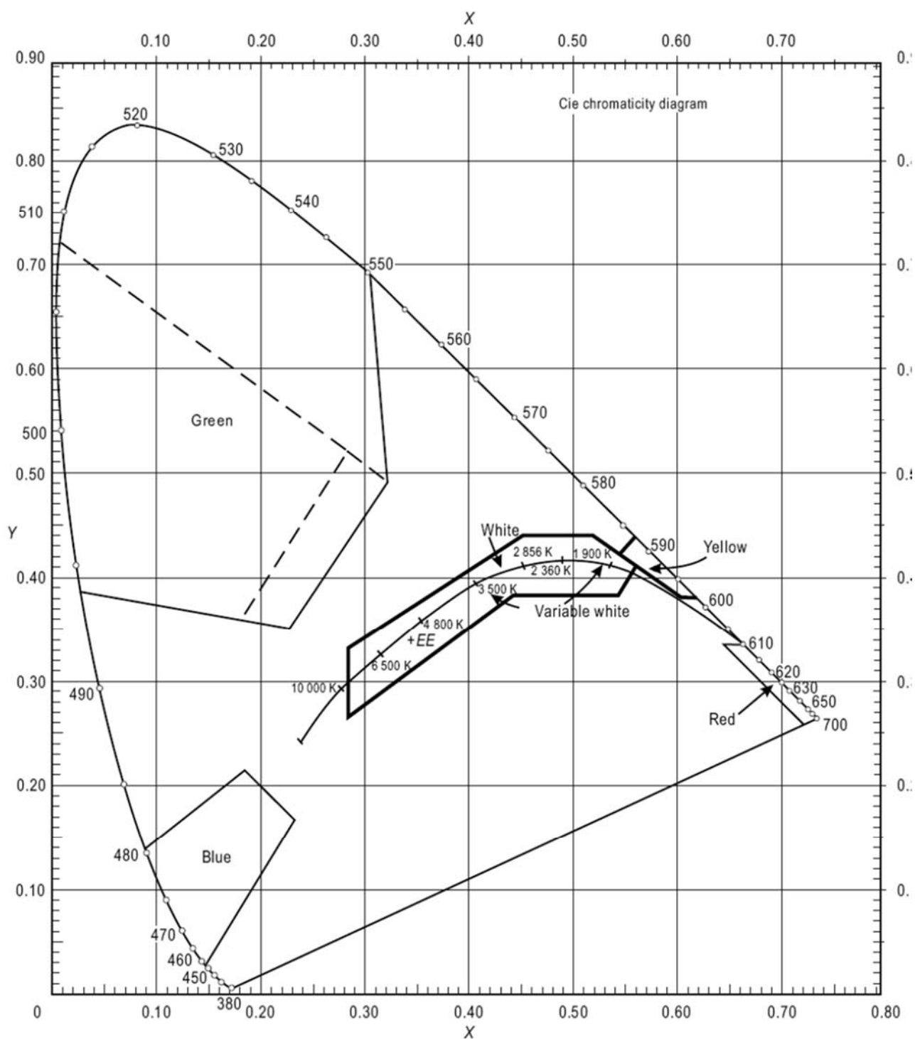
Figure A1-I Colours for aeronautical ground lights
