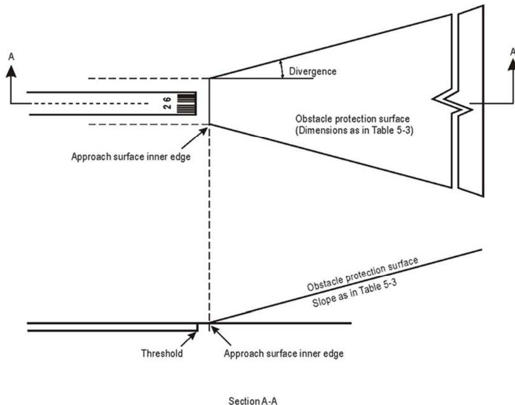
Figure 5-21 Obstacle protection surface for visual approach slope indicator system
