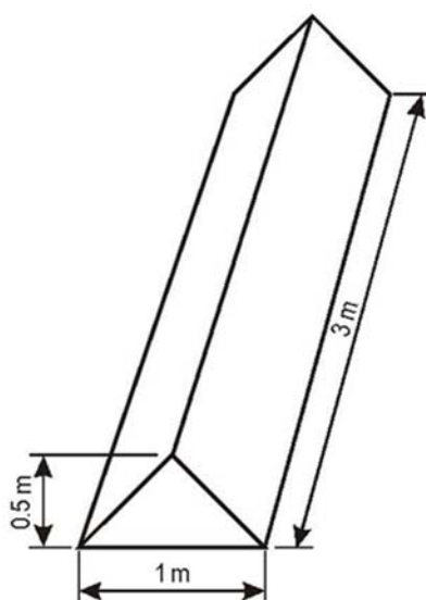
Figure 5-34 Boundary markers
