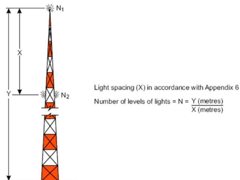
Figure 6-2 Examples of marking and lighting of tall structures
