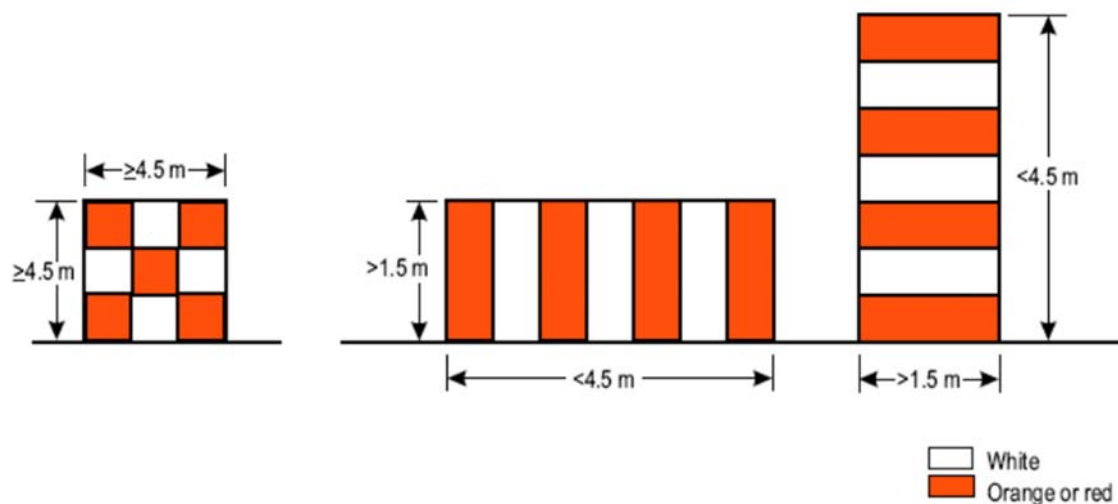
Figure 6-1 Basic marking patterns
