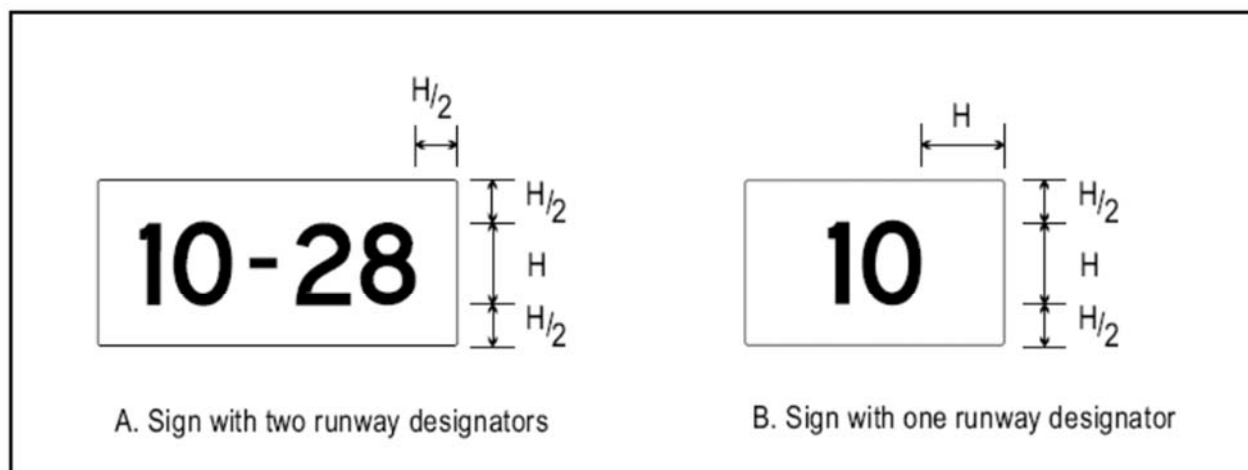
Figure A4-3. Sign dimensions
