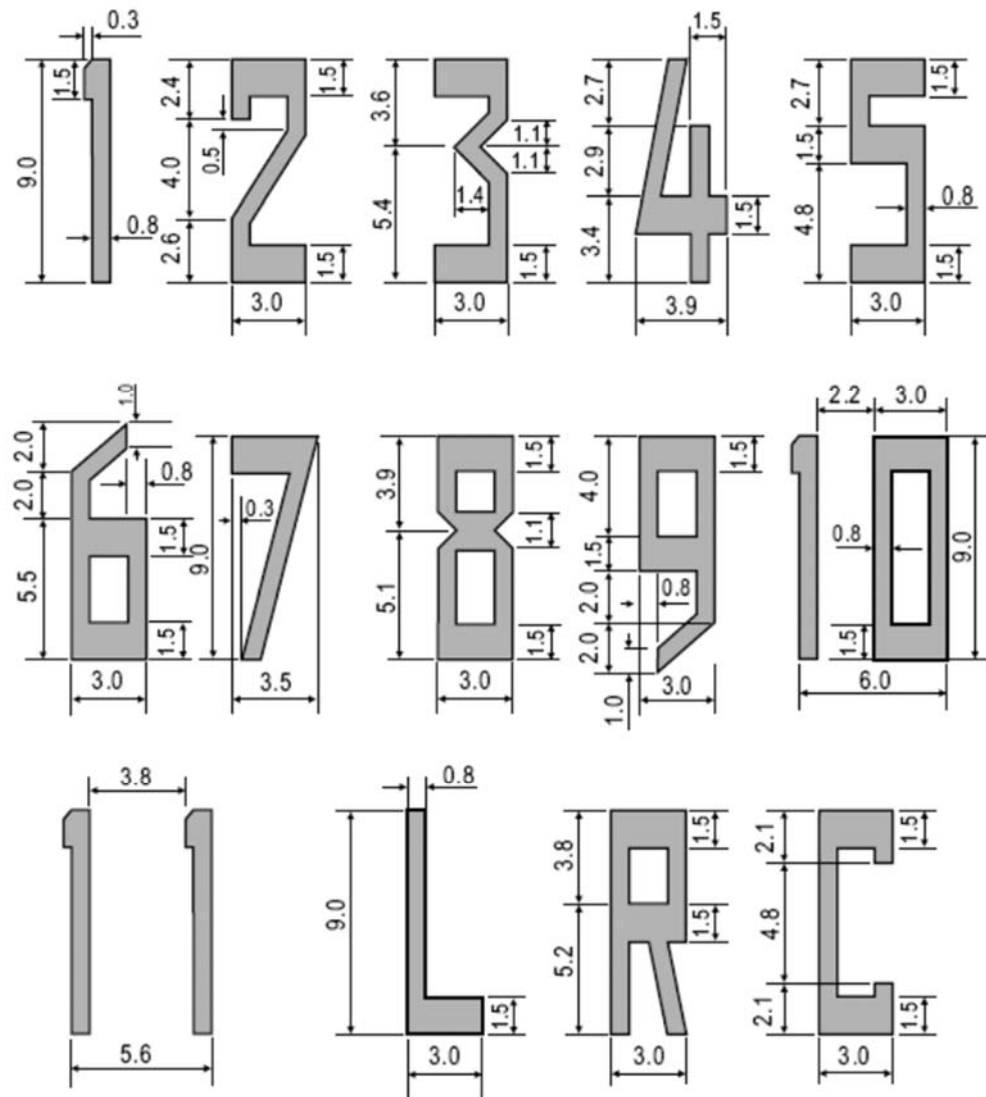
Figure 5-3 Form and proportions of numbers and letters for runway designation markings
