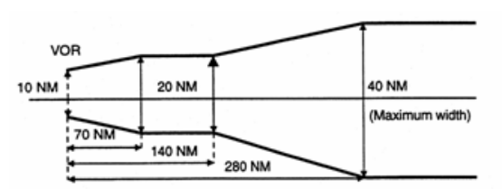
Figure 1: Corridor width from a VOR station
