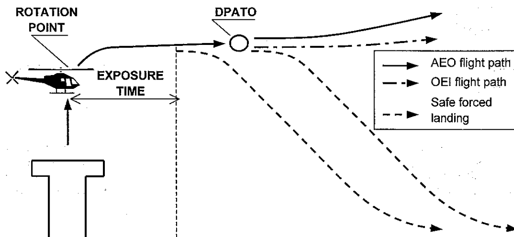
Figure 2: Typical take-off profile PC2 from a helideck/elevated FATO with exposure time, non-hostile environment
