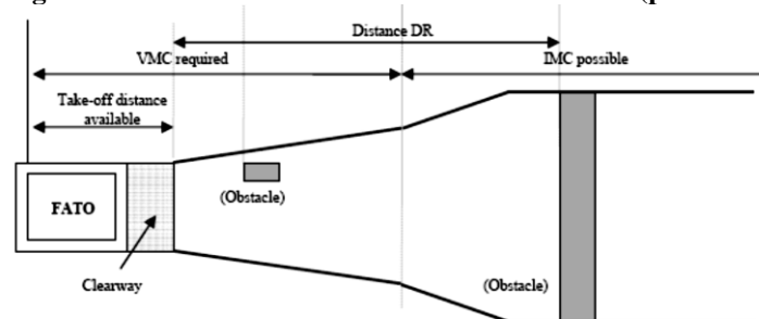
Figure 4: Performance Class 2 Obstacle Clearance (plan view)
