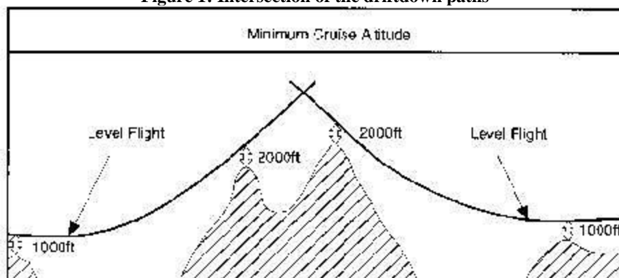
Figure 1: Intersection of the driftdown paths
