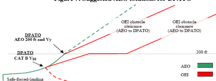
Figure 7: Suggested AEO locations for DPATO
