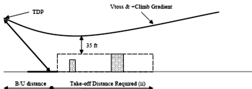
Figure 3: Helipad take-off
