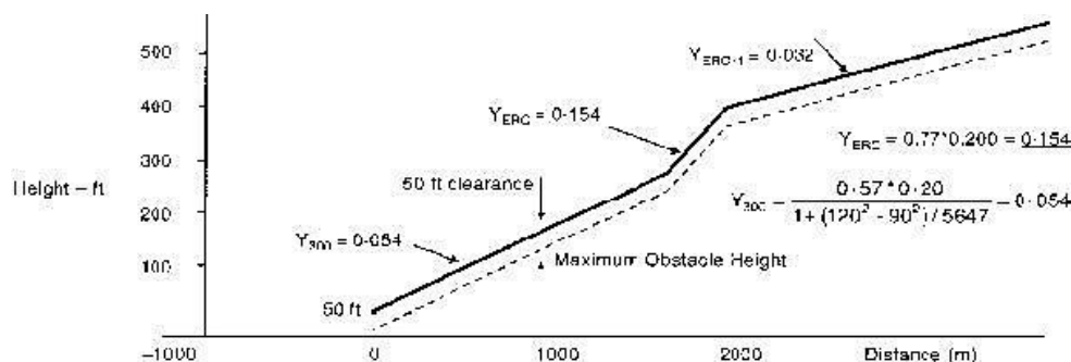
Figure 3: Assumed engine failure height less than 200 ft
