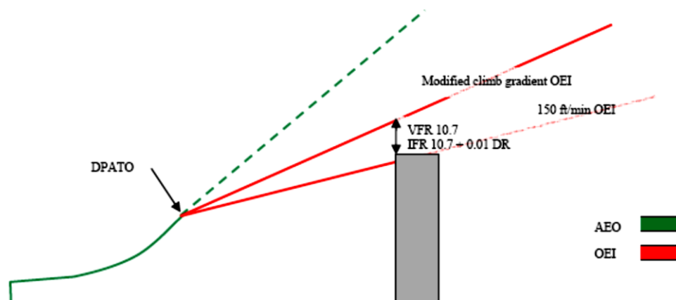
Figure 6: Performance Class 2 (enhanced climb gradient)
