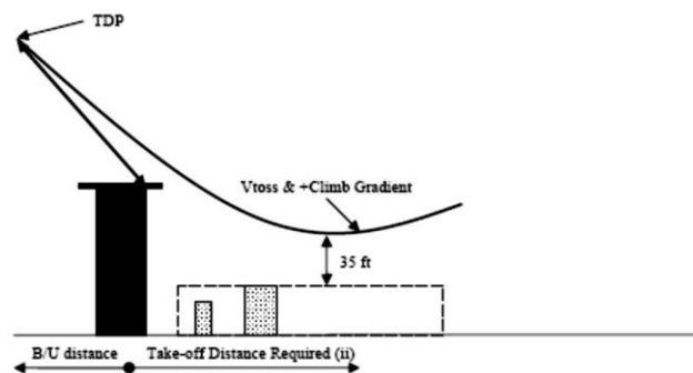
Figure 4: Elevate Helipad take – off
