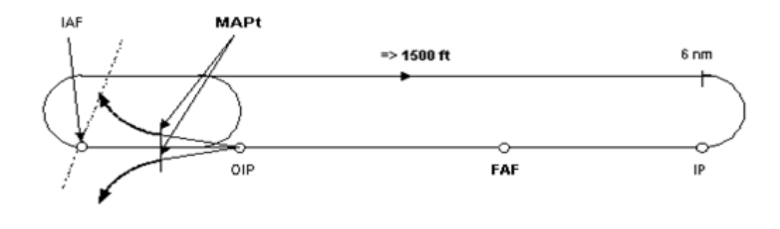
Figure 3: Holding pattern & race track procedure
