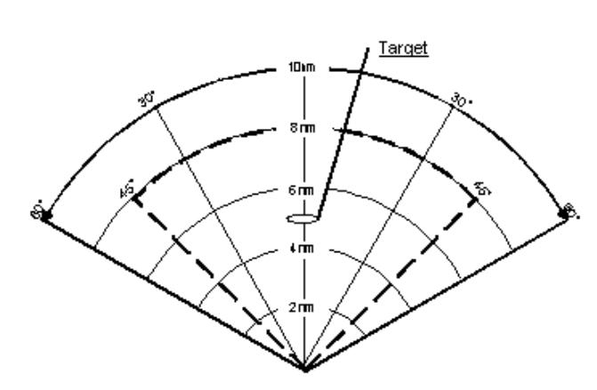
Figure 5: Missed approach area left & right
