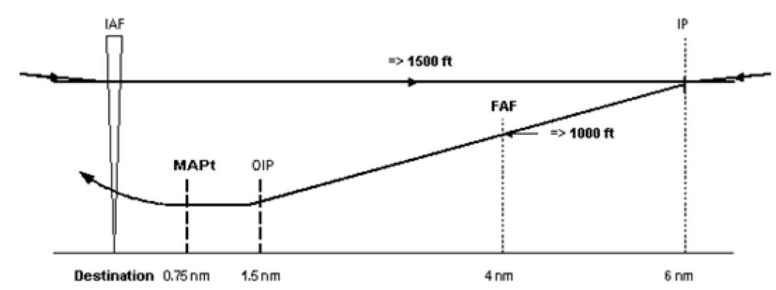
Figure 4: Vertical profile
