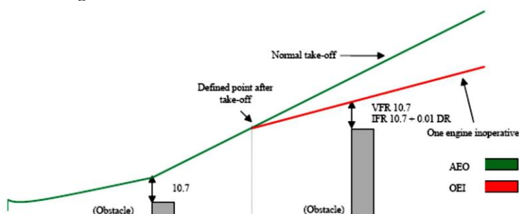
Figure 3: Performance Class 2 Obstacle Clearance
