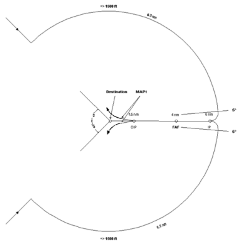
Figure 1: Arc procedure
