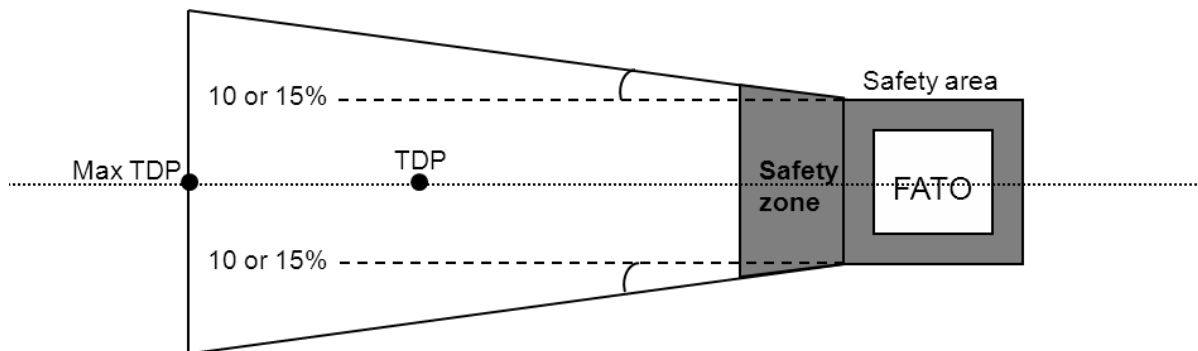
Figure 2: Obstacle accountability
