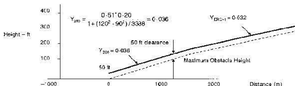
Figure 2: Assumed engine failure height 200 ft
