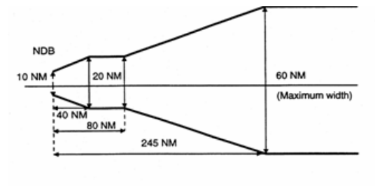
Figure 2: Corridor width from an NDB
